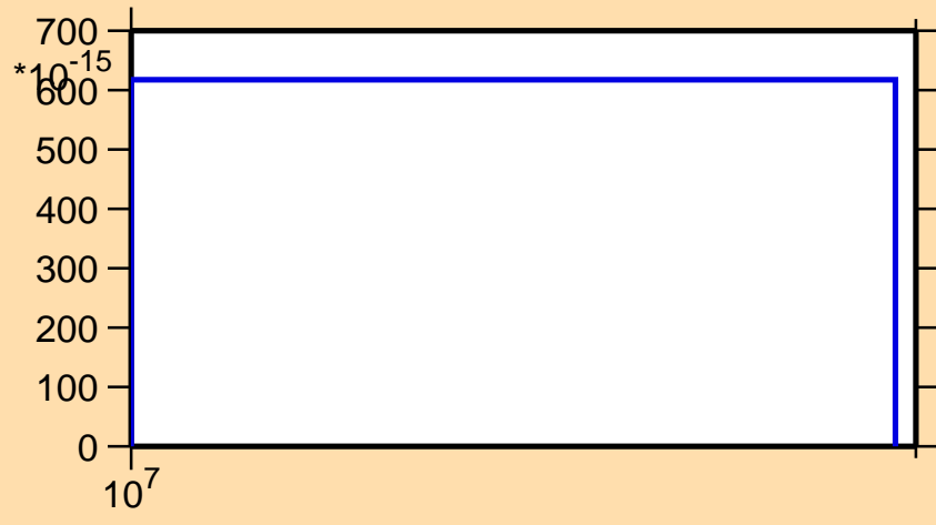
\sigma vs. E for ^{230}\text{Pa}(n,p\alpha)
