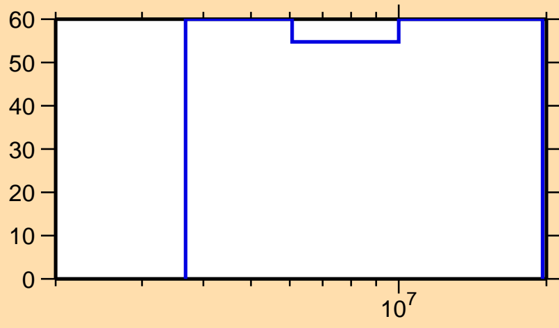
\Delta\sigma/\sigma vs. E for ^{230}\text{Pa}(n,2n)
