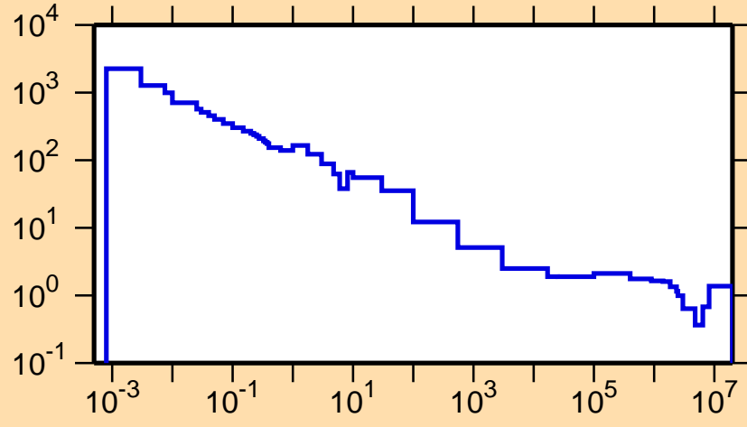
\sigma vs. E for ^{230}\text{Pa}(n,f)
