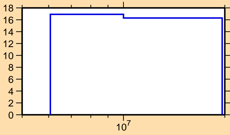
\Delta\sigma/\sigma vs. E for ^{231}\text{Pa}(n,2n)
