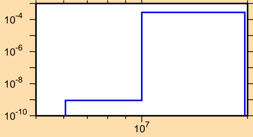
\sigma vs. E for ^{231}\text{Pa}(n,np)
