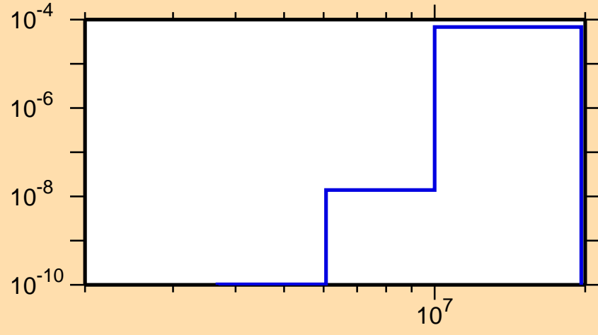
\sigma vs. E for ^{231}\text{Pa}(n,n\alpha)
