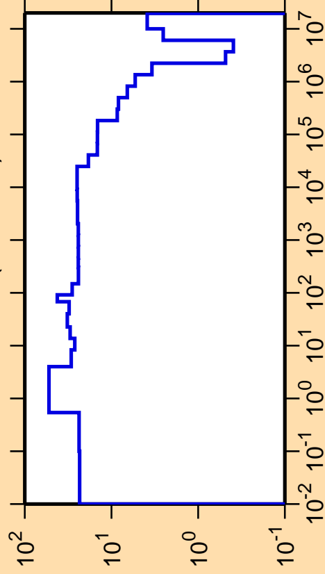
\Delta\sigma/\sigma vs. E for ^{231}\text{Pa}(n,\text{nonel.})
