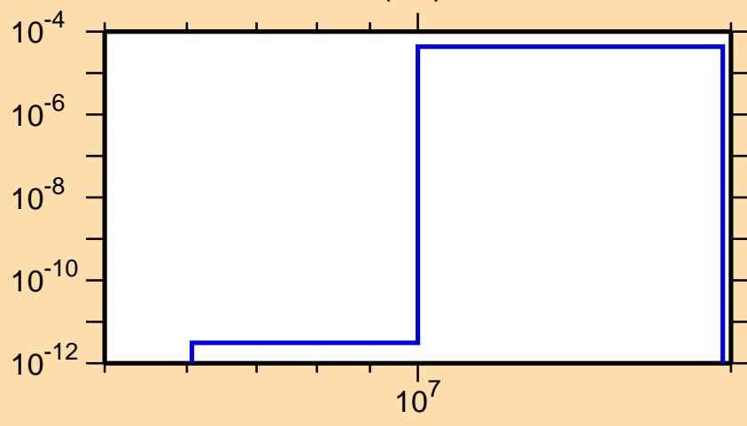
\sigma vs. E for ^{231}\text{Pa}(n,t)
