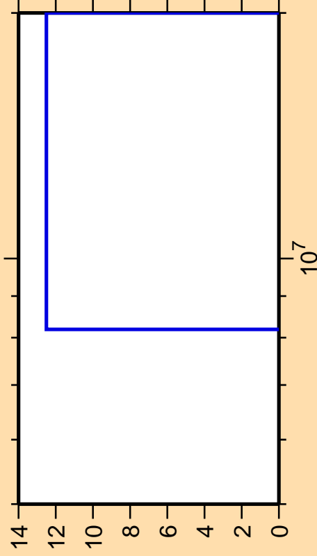
\Delta\sigma/\sigma vs. E for ^{231}\text{Pa}(n,2n\alpha)
