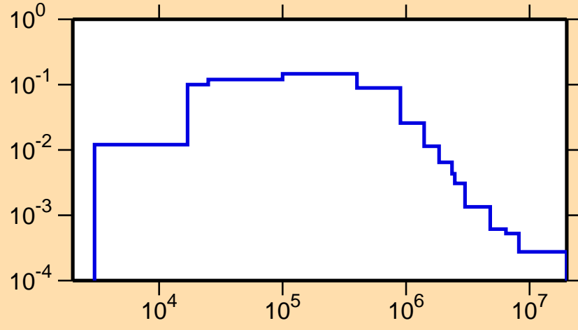
\sigma vs. E for ^{231}\text{Pa}(n,n_1)
