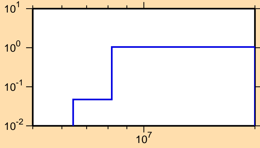
\sigma vs. E for ^{231}\text{Pa}(n,2n)
