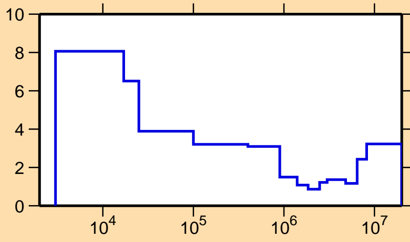
\Delta\sigma/\sigma vs. E for ^{231}\text{Pa}(n,\text{el.})
