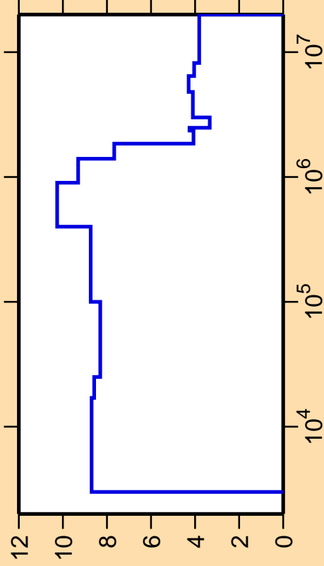
\Delta\sigma/\sigma vs. E for ^{231}\text{Pa}(n,n_1)
