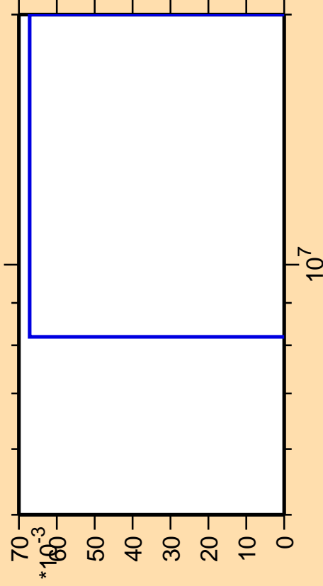
\Delta\sigma/\sigma vs. E for ^{231}\text{Pa}(n,\text{He}3)
