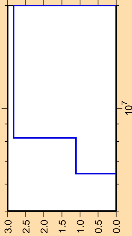
\Delta\sigma/\sigma vs. E for ^{231}\text{Pa}(n,d)
