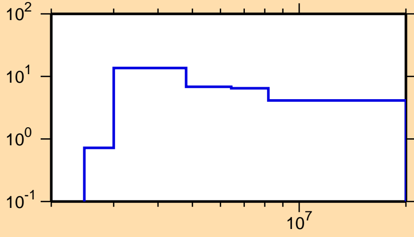
\Delta\sigma/\sigma vs. E for ^{231}\text{Pa}(n,p)
