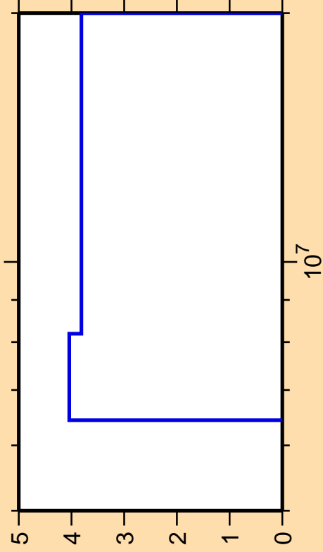
\Delta\sigma/\sigma vs. E for ^{231}\text{Pa}(n,n_1)
