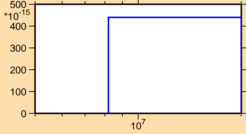
\sigma vs. E for ^{231}\text{Pa}(n,\text{He}3)
