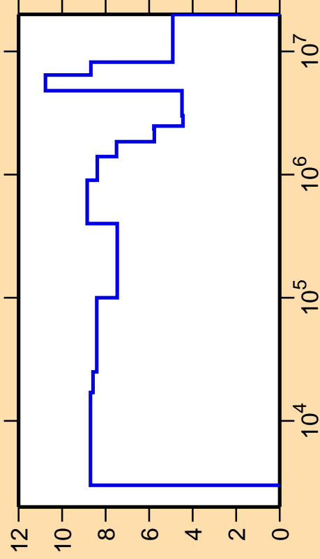
\Delta\sigma/\sigma vs. E for ^{231}\text{Pa}(n,\text{inel.})
