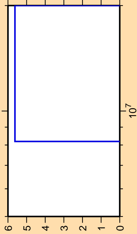
\Delta\sigma/\sigma vs. E for ^{231}\text{Pa}(n,\text{nd})
