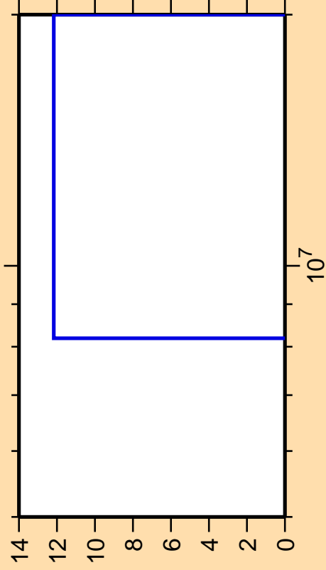
\Delta\sigma/\sigma vs. E for ^{231}\text{Pa}(n,2np)
