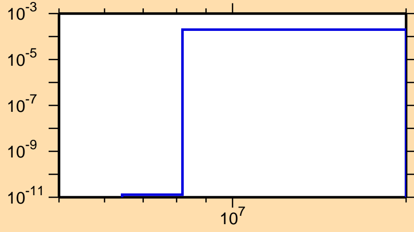
\sigma vs. E for ^{231}\text{Pa}(n,d)
