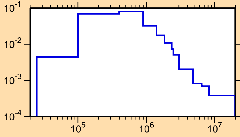
\sigma vs. E for ^{231}\text{Pa}(n,n_2)
