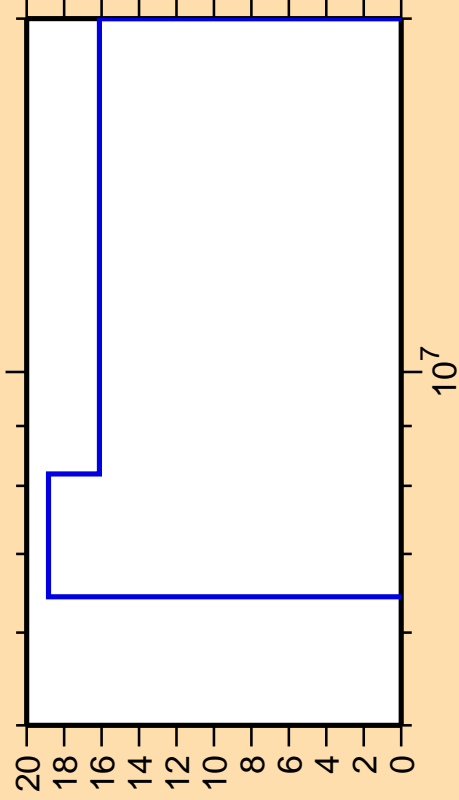
\Delta\sigma/\sigma vs. E for ^{231}\text{Pa}(n,2n)
