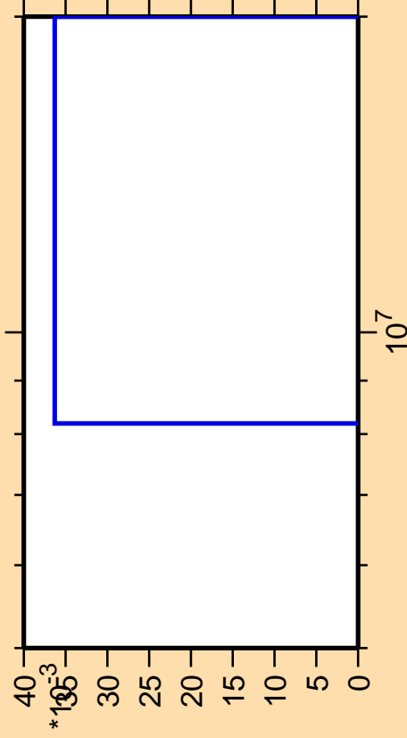
\Delta\sigma/\sigma vs. E for ^{231}\text{Pa}(n,3n\alpha)
