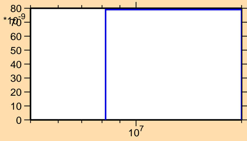
\sigma vs. E for ^{231}\text{Pa}(n,nt)
