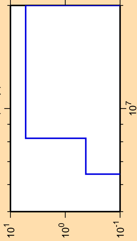
\Delta\sigma/\sigma vs. E for ^{231}\text{Pa}(n,np)
