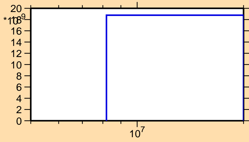
\sigma vs. E for ^{231}\text{Pa}(n,2n\alpha)
