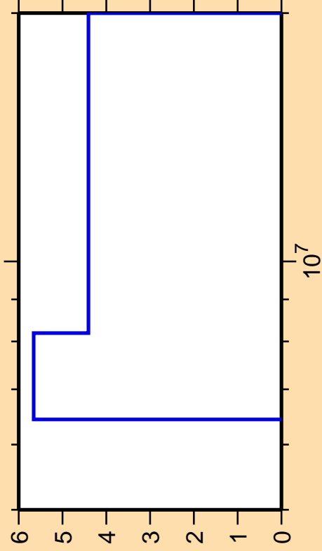
\Delta\sigma/\sigma vs. E for ^{231}\text{Pa}(n,f)
