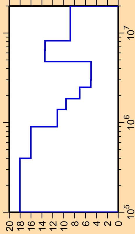
\Delta\sigma/\sigma vs. E for ^{231}\text{Pa}(n,\text{ncont.})
