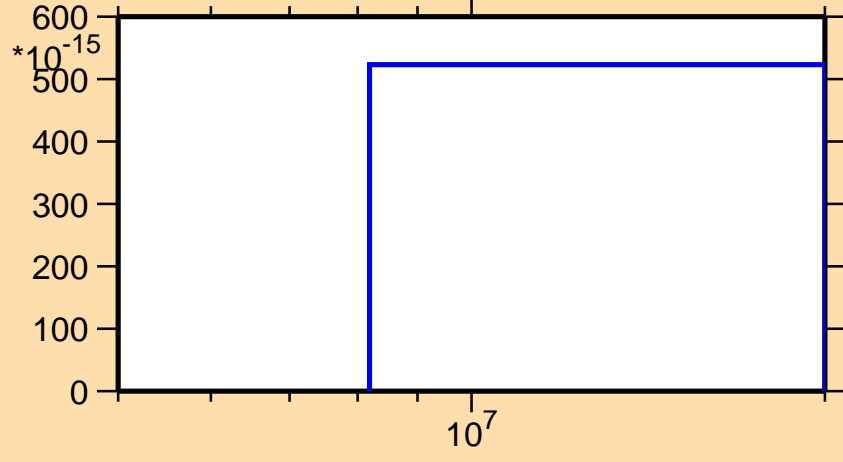
\sigma vs. E for ^{231}\text{Pa}(n,3n\alpha)
