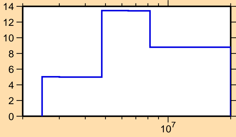
\Delta\sigma/\sigma vs. E for ^{231}\text{Pa}(n,n\text{cont.})
