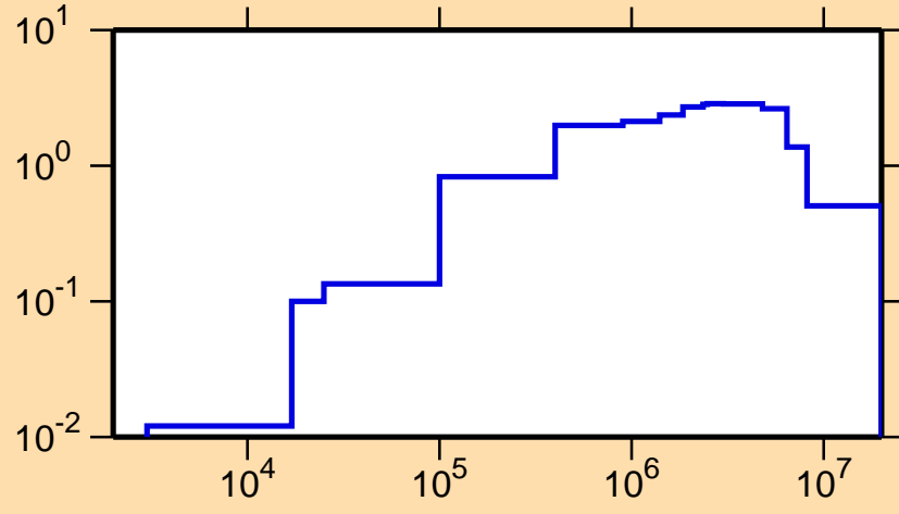
\sigma vs. E for ^{231}\text{Pa}(n,\text{inel.})
