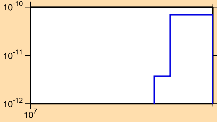
\sigma vs. E for ^{232}\text{Pa}(n,\text{He3})
