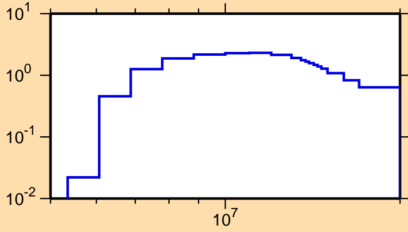
\sigma vs. E for ^{232}\text{Pa}(n,2n)
