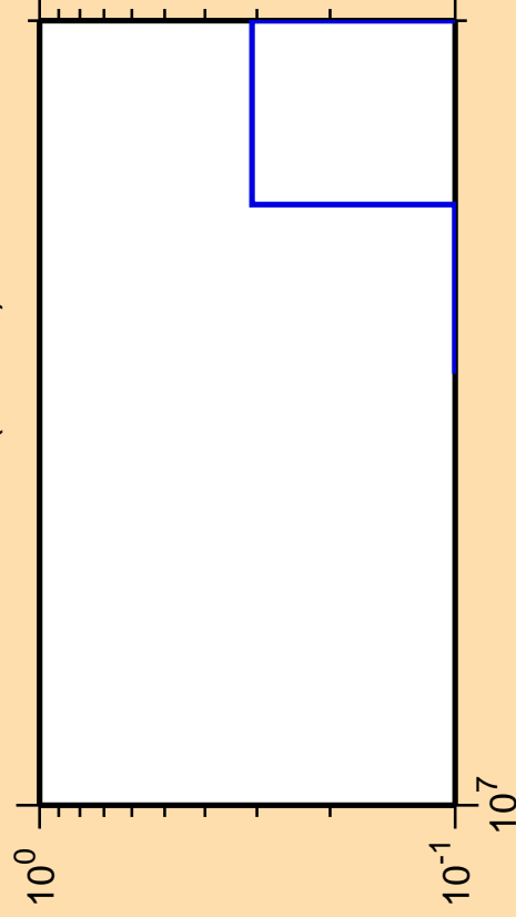
\Delta\sigma/\sigma vs. E for ^{232}\text{Pa} (mt 11)
