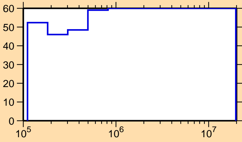
\Delta\sigma/\sigma vs. E for ^{232}\text{Pa}(n,f)
