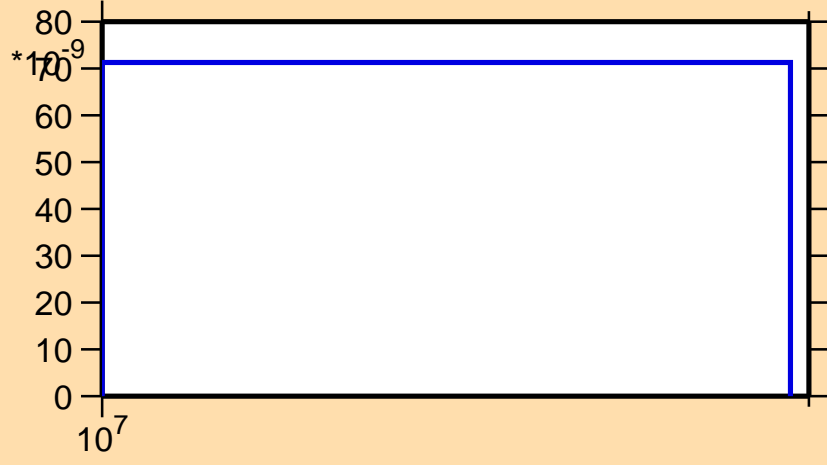
\sigma vs. E for ^{232}\text{Pa}(n,nt)
