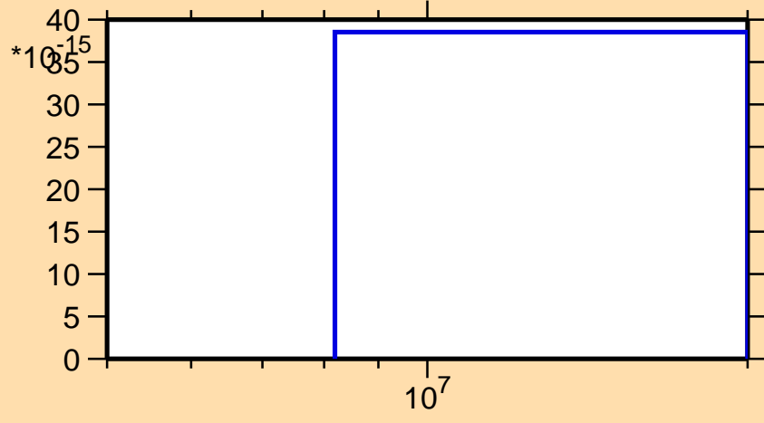
\sigma vs. E for ^{232}\text{Pa}(n,3n\alpha)
