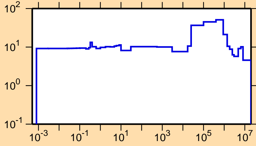
\Delta\sigma/\sigma vs. E for ^{232}\text{Pa}(n,el.)
