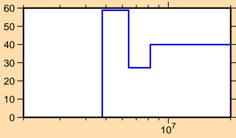
\Delta\sigma/\sigma vs. E for ^{232}\text{Pa}(n,2n)
