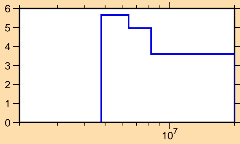
\Delta\sigma/\sigma vs. E for ^{232}\text{Pa}(n,\text{tot.})
