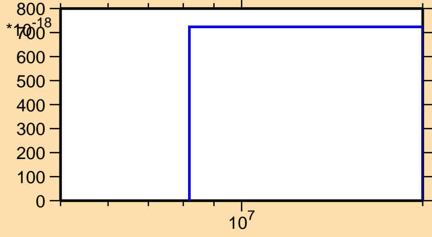
\sigma vs. E for ^{232}\text{Pa} (mt 11)
