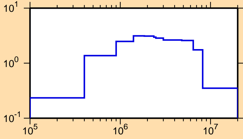
\sigma vs. E for ^{232}\text{Pa}(n,\text{inel.})
