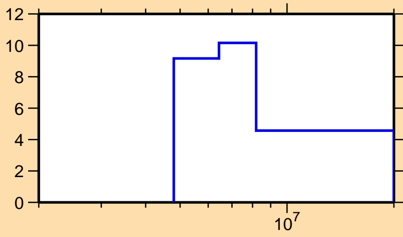
\Delta\sigma/\sigma vs. E for ^{232}\text{Pa}(n,\text{el.})
