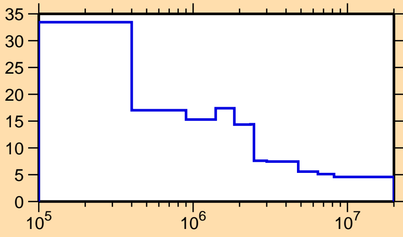
\Delta\sigma/\sigma vs. E for ^{232}\text{Pa}(n,\text{nonel.})
