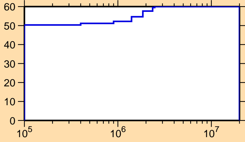
\Delta\sigma/\sigma vs. E for ^{232}\text{Pa}(n,n_1)
