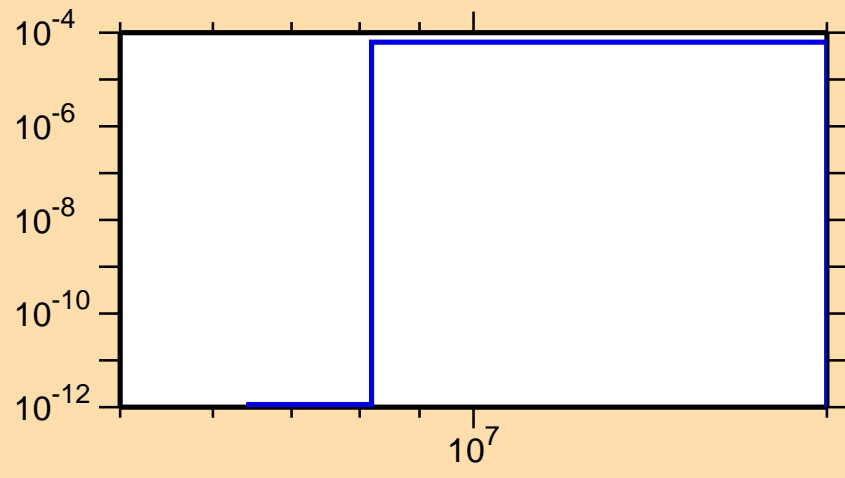
\sigma vs. E for ^{232}\text{Pa}(n,t)
