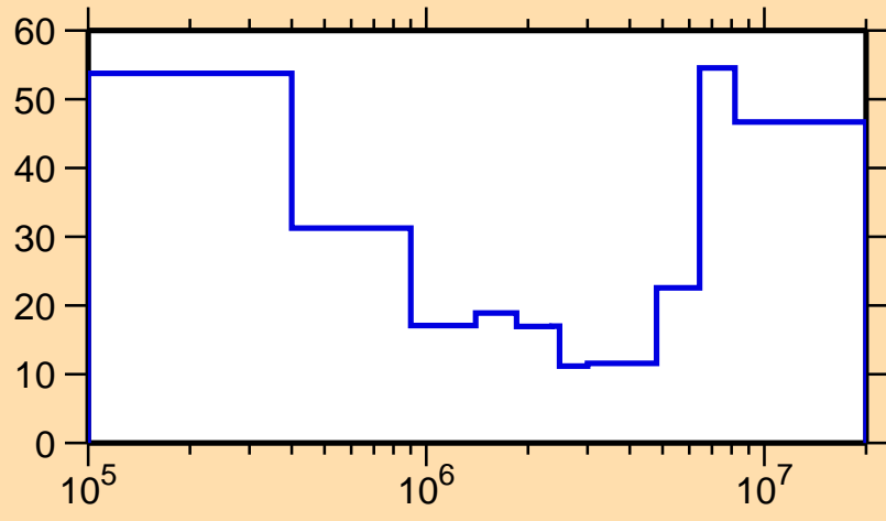
\Delta\sigma/\sigma vs. E for ^{232}\text{Pa}(n,n\text{cont.})
