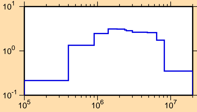
\sigma vs. E for ^{232}\text{Pa}(n,n\text{cont.})
