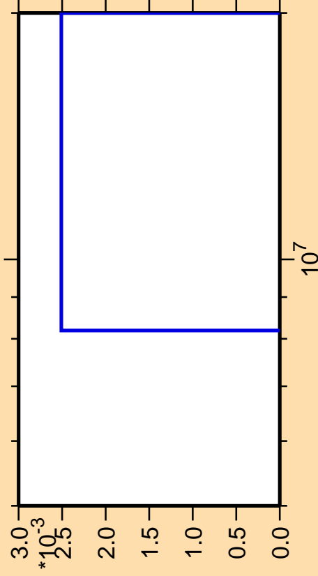
\Delta\sigma/\sigma vs. E for ^{232}\text{Pa} (mt 11)
