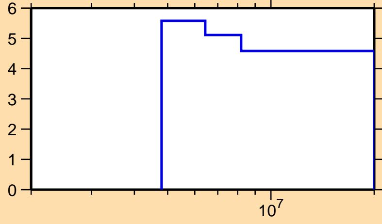
\Delta\sigma/\sigma vs. E for ^{232}\text{Pa}(n,\text{nonel.})
