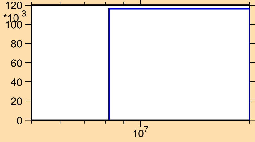
\sigma vs. E for ^{232}\text{Pa}(n,3n)
