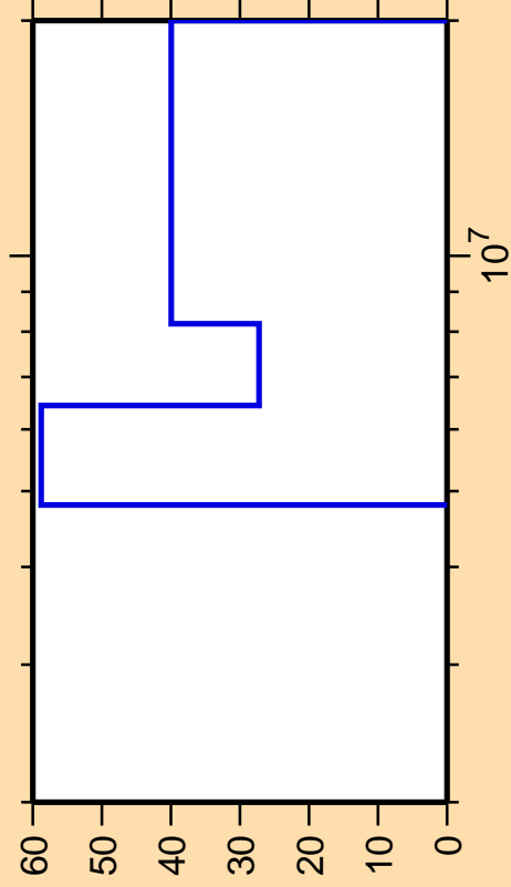
\Delta\sigma/\sigma vs. E for ^{232}\text{Pa}(n,2n)
