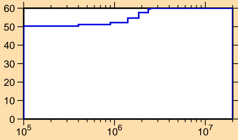
\Delta\sigma/\sigma vs. E for ^{232}\text{Pa}(n,n_1)
