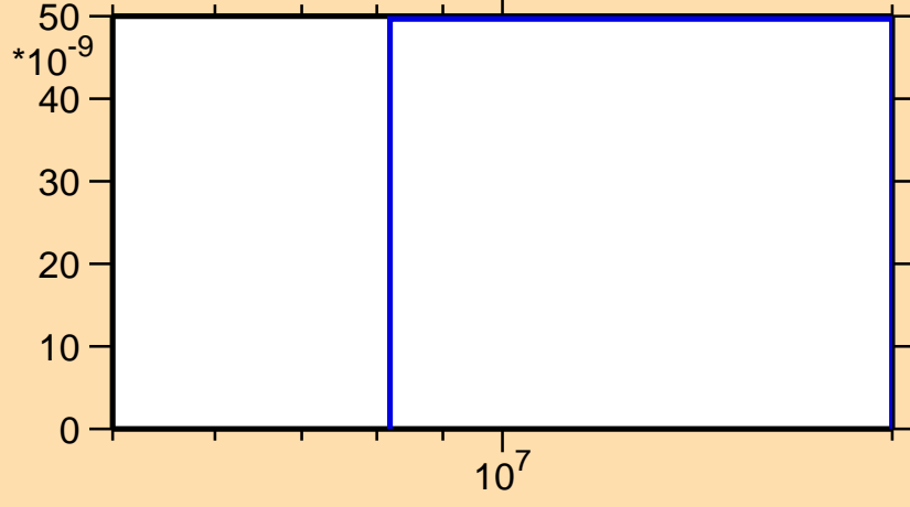
\sigma vs. E for ^{232}\text{Pa}(n,2np)
