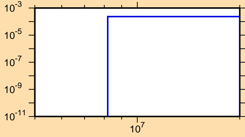
\sigma vs. E for ^{232}\text{Pa}(n,d)
