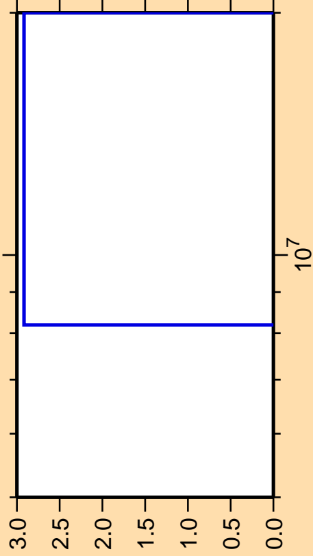
\Delta\sigma/\sigma vs. E for ^{232}\text{Pa}(n,\text{He}3)
