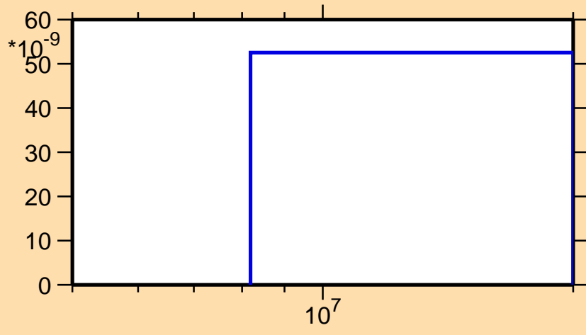
\sigma vs. E for ^{232}\text{Pa}(n,2n\alpha)
