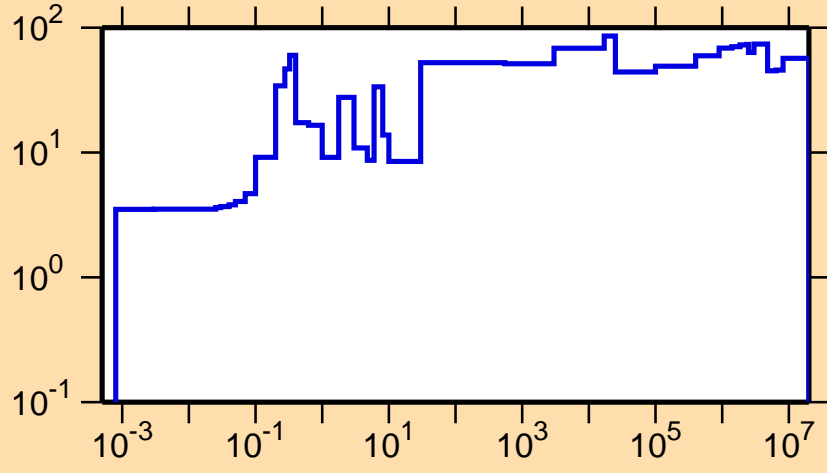
\Delta\sigma/\sigma vs. E for ^{232}\text{Pa}(n,\gamma)
