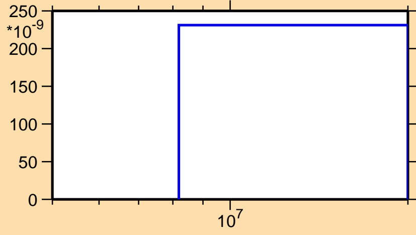
\sigma vs. E for ^{232}\text{Pa}(n,\text{nd})
