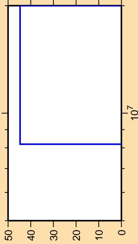
\Delta\sigma/\sigma vs. E for ^{232}\text{Pa}(n,\text{nd})
