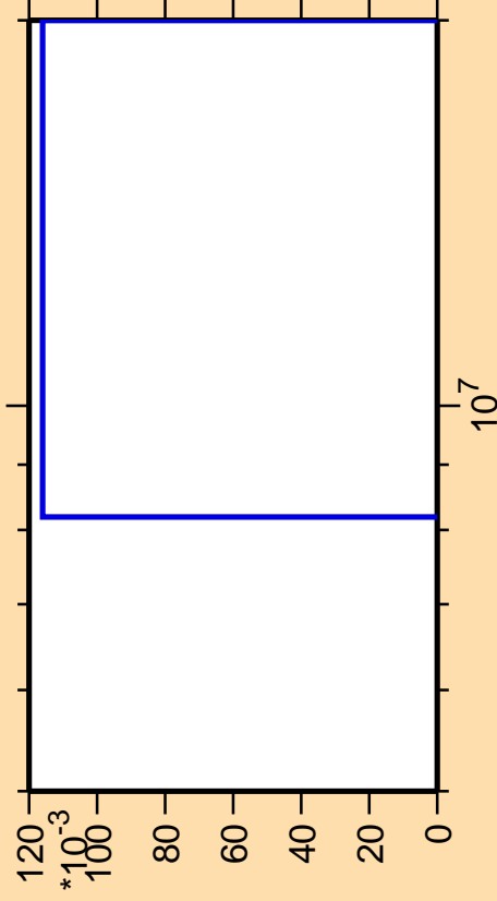
\Delta\sigma/\sigma vs. E for ^{232}\text{Pa}(n,3n\alpha)
