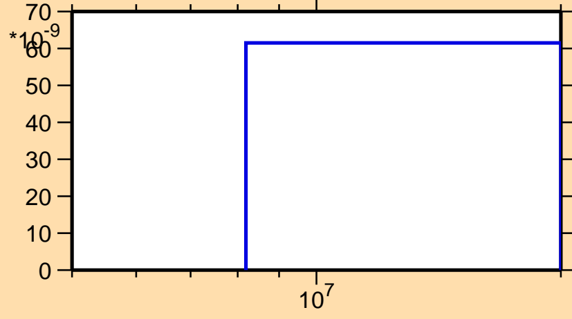
\sigma vs. E for ^{232}\text{Pa}(n,nt)
