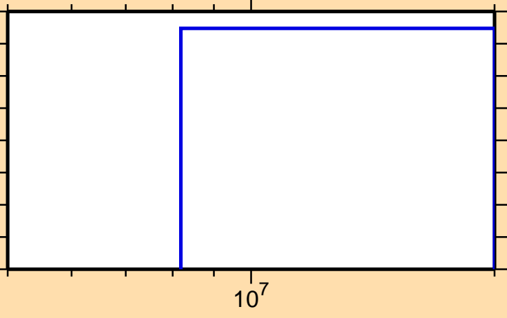
\sigma vs. E for ^{232}\text{Pa}(n,\text{He}3)
