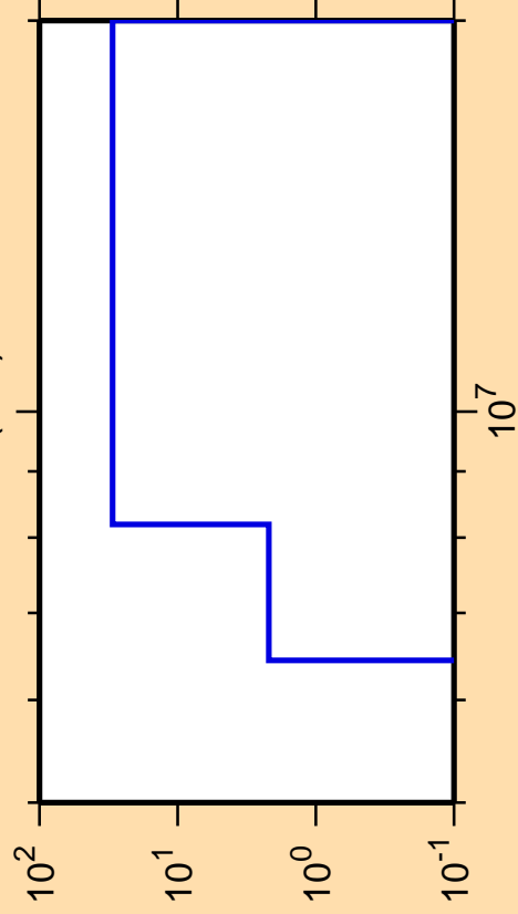
\Delta\sigma/\sigma vs. E for ^{232}\text{Pa}(n,d)
