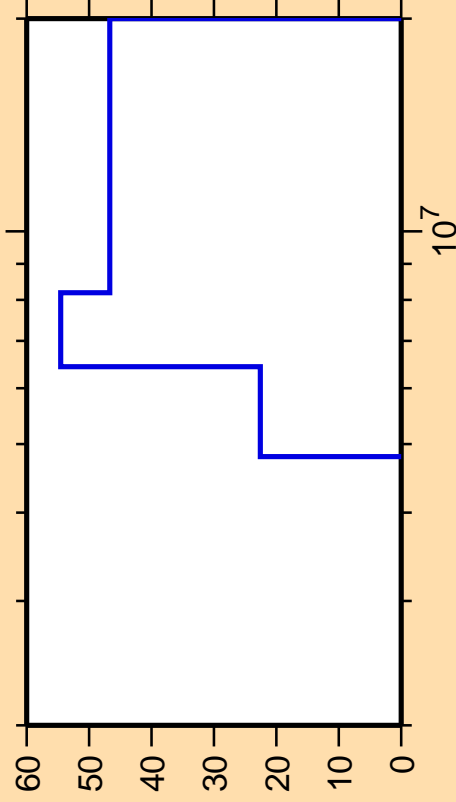
\Delta\sigma/\sigma vs. E for ^{232}\text{Pa}(n,n\text{cont.})
