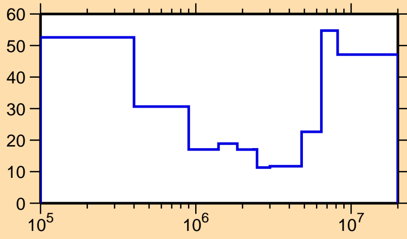
\Delta\sigma/\sigma vs. E for ^{232}\text{Pa}(n,\text{inel.})
