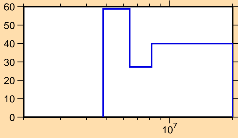
\Delta\sigma/\sigma vs. E for ^{232}\text{Pa}(n,2n)
