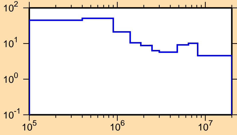
\Delta\sigma/\sigma vs. E for ^{232}\text{Pa}(n,\text{el.})
