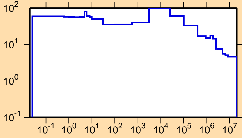
\Delta\sigma/\sigma vs. E for ^{232}\text{Pa}(n,\text{nonel.})
