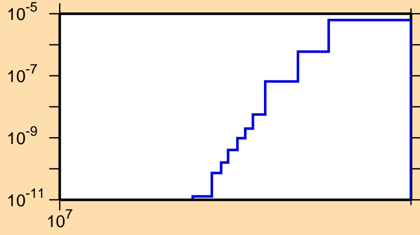
\sigma vs. E for ^{234}\text{Pa}(n,nd)
