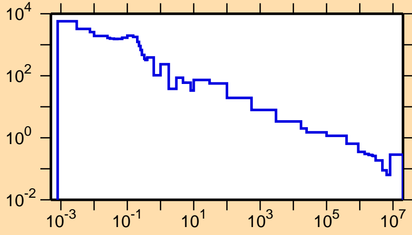
\sigma vs. E for ^{234}\text{Pa}(n,f)
