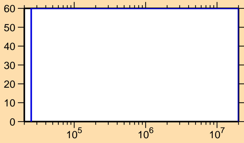
\Delta\sigma/\sigma vs. E for ^{234}\text{Pa}(n,n_1)
