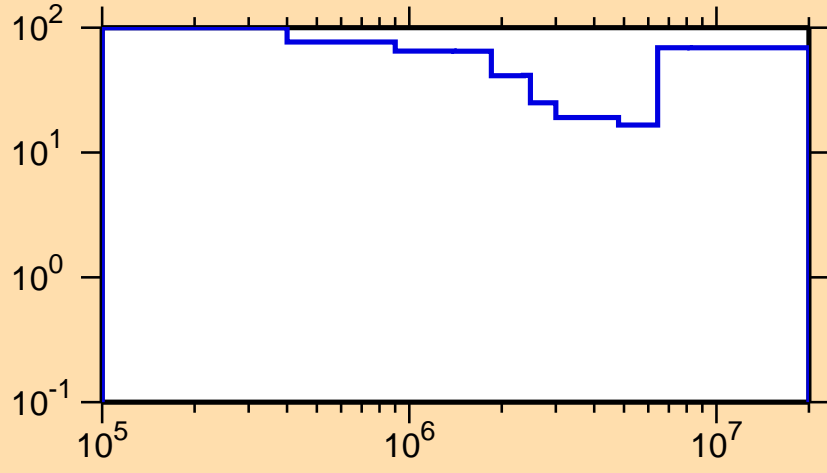
\Delta\sigma/\sigma vs. E for ^{234}\text{Pa}(n,n\text{cont.})
