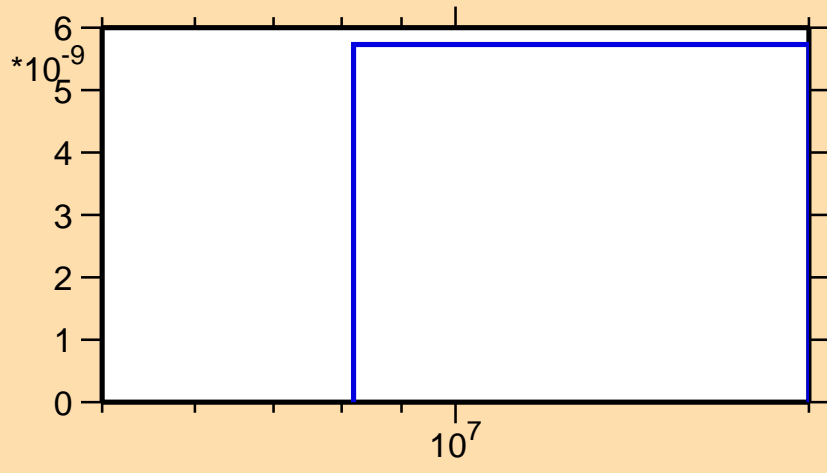
\sigma vs. E for ^{234}\text{Pa}(n,2n\alpha)
