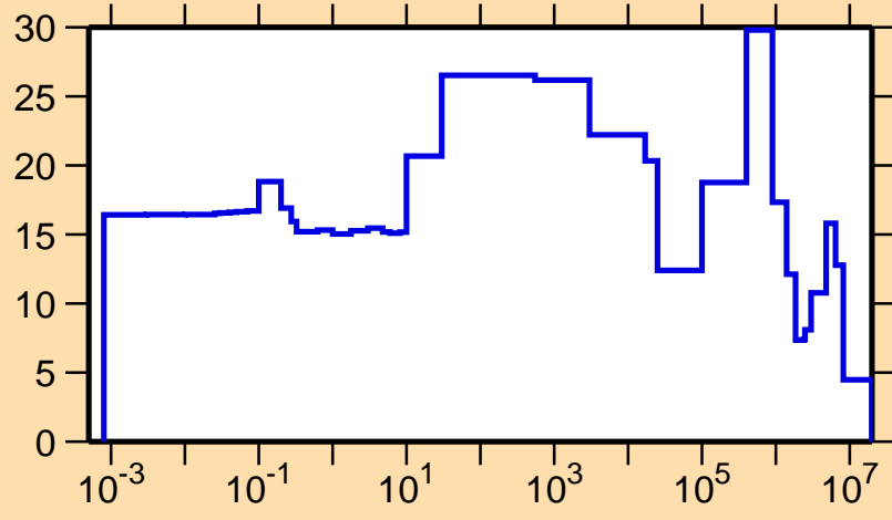
\Delta\sigma/\sigma vs. E for ^{234}\text{Pa}(n,el.)
