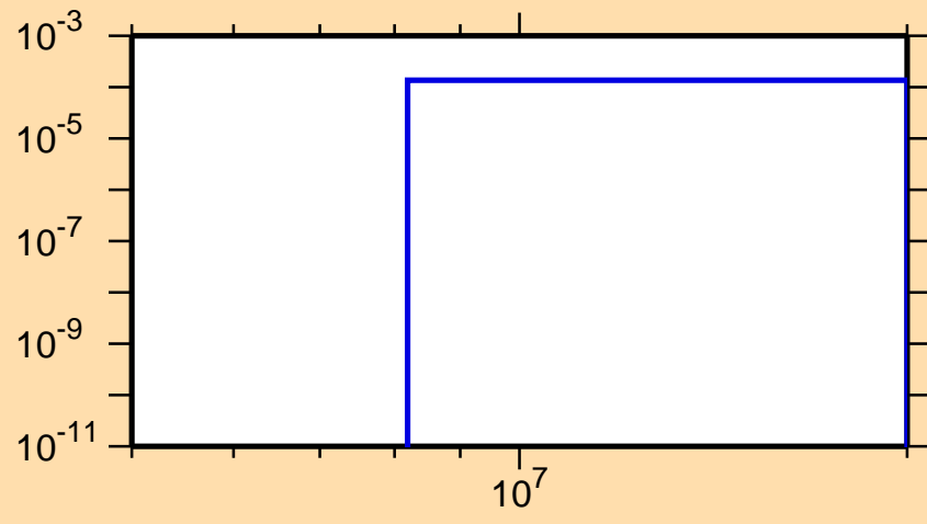
\sigma vs. E for ^{234}\text{Pa}(n,d)
