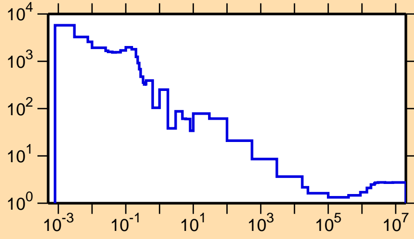
\sigma vs. E for ^{234}\text{Pa}(n,\text{nonel.})
