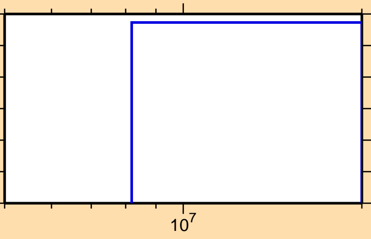
\sigma vs. E for ^{234}\text{Pa}(n,2n\alpha)
