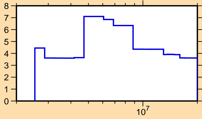
\Delta\sigma/\sigma vs. E for ^{234}\text{Pa}(n,\text{tot.})
