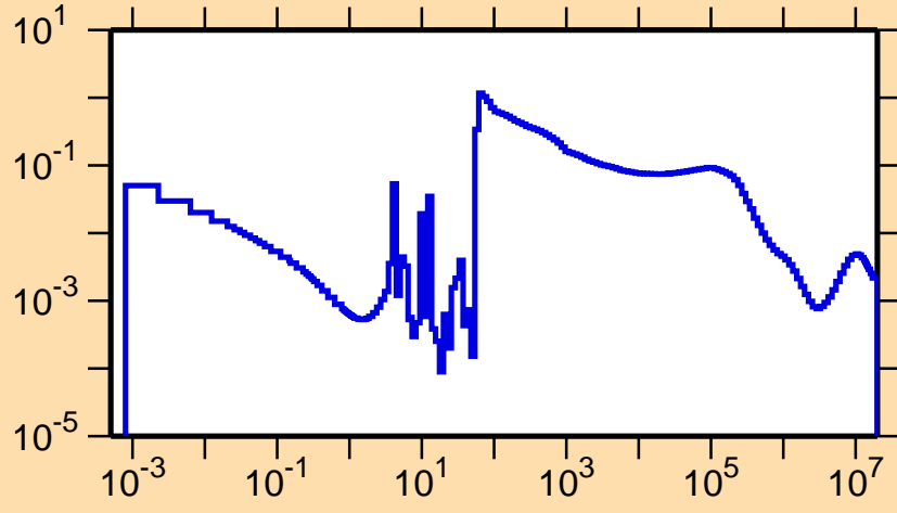
\sigma vs. E for ^{234}\text{Pa}(n,\gamma)
