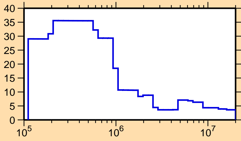
\Delta\sigma/\sigma vs. E for ^{234}\text{Pa}(n, tot.)
