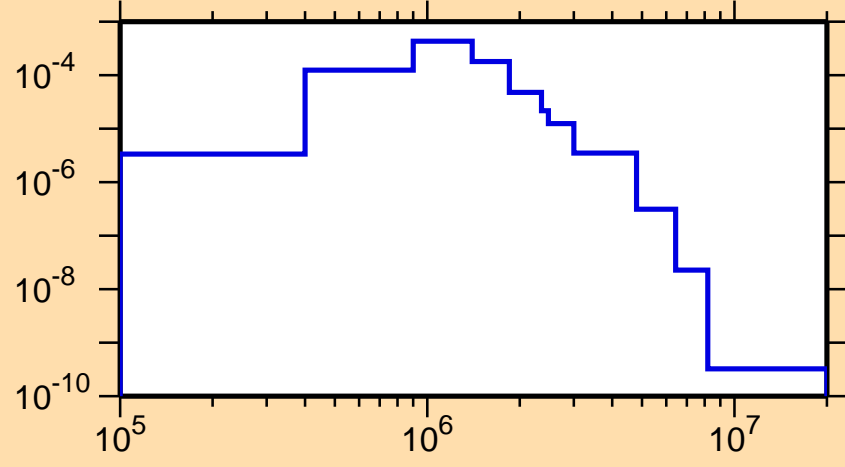
\sigma vs. E for ^{234}\text{Pa}(n,n_4)
