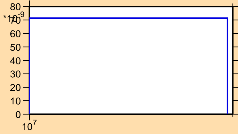
\sigma vs. E for ^{235}\text{Pa}(n,2n\alpha)
