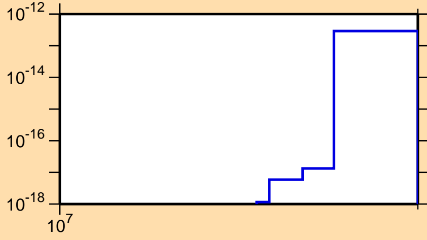
\sigma vs. E for ^{236}\text{Pa}(\text{mt } 11)
