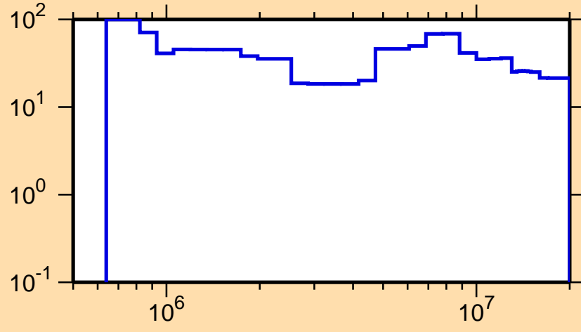
\Delta\sigma/\sigma vs. E for ^{236}\text{Pa}(n,n\text{cont.})
