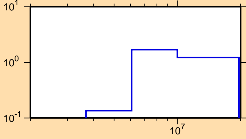
\sigma vs. E for ^{236}\text{Pa}(n,2n)
