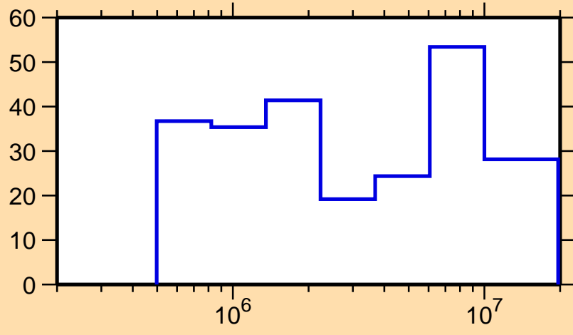
\Delta\sigma/\sigma vs. E for ^{236}\text{Pa}(n,\text{inel.})
