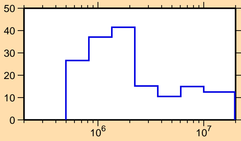
\Delta\sigma/\sigma vs. E for ^{236}\text{Pa}(n,\text{nonel.})
