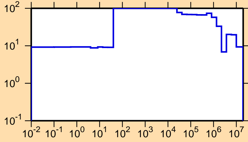
\Delta\sigma/\sigma vs. E for ^{236}\text{Pa}(n,el.)
