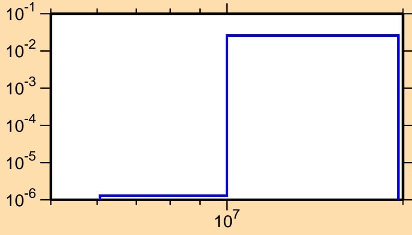
\sigma vs. E for ^{236}\text{Pa}(n,n\alpha)
