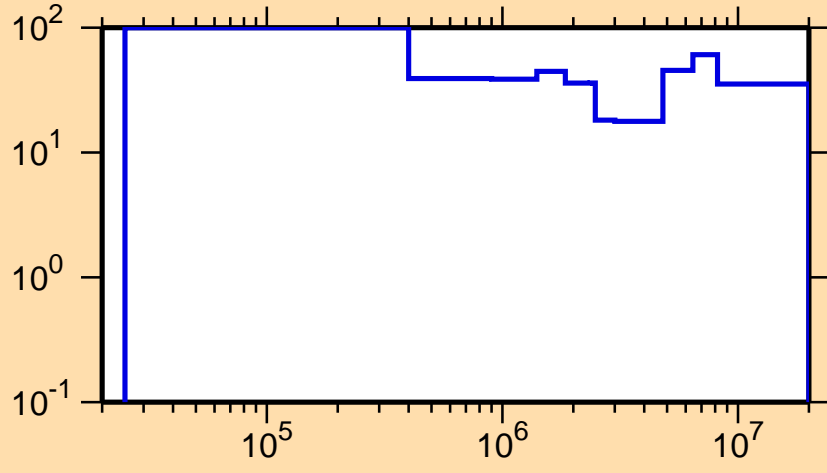
\Delta\sigma/\sigma vs. E for ^{236}\text{Pa}(n,\text{inel.})
