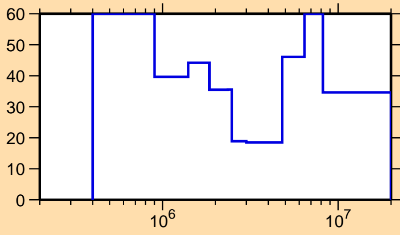
\Delta\sigma/\sigma vs. E for ^{236}\text{Pa}(n,n\text{cont.})
