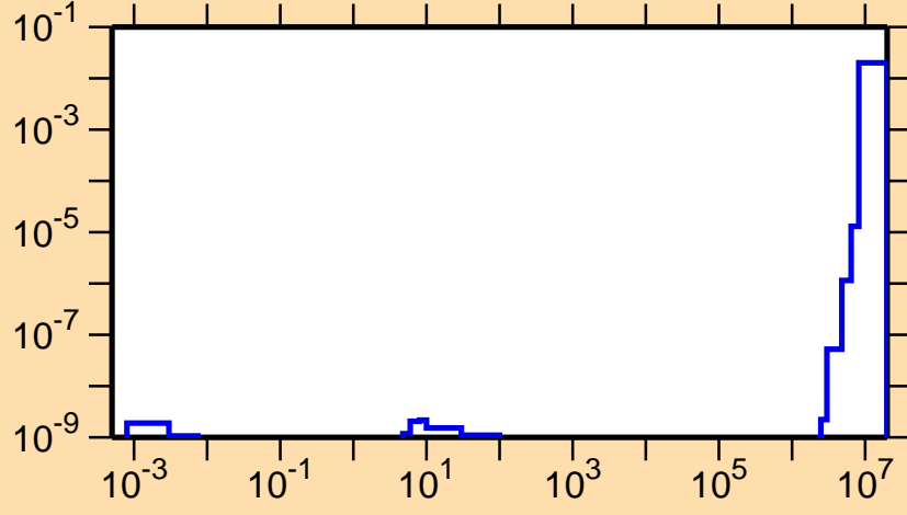
\sigma vs. E for ^{236}\text{Pa}(n,\alpha)
