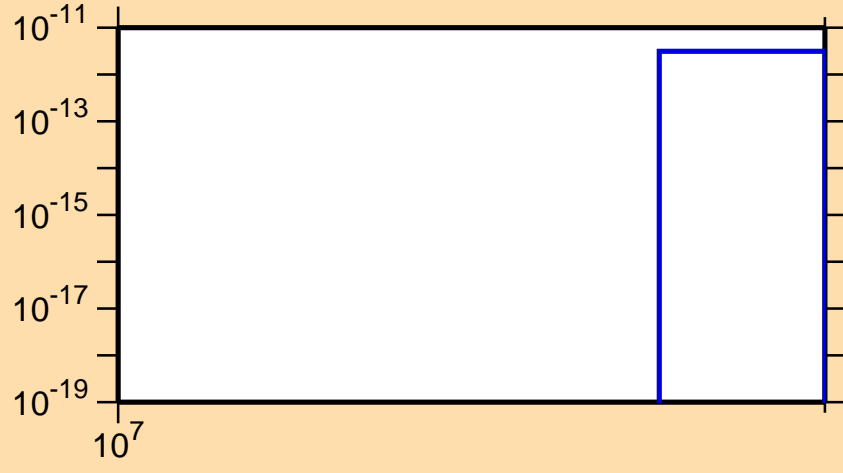
\sigma vs. E for ^{237}\text{Pa} (mt 11)
