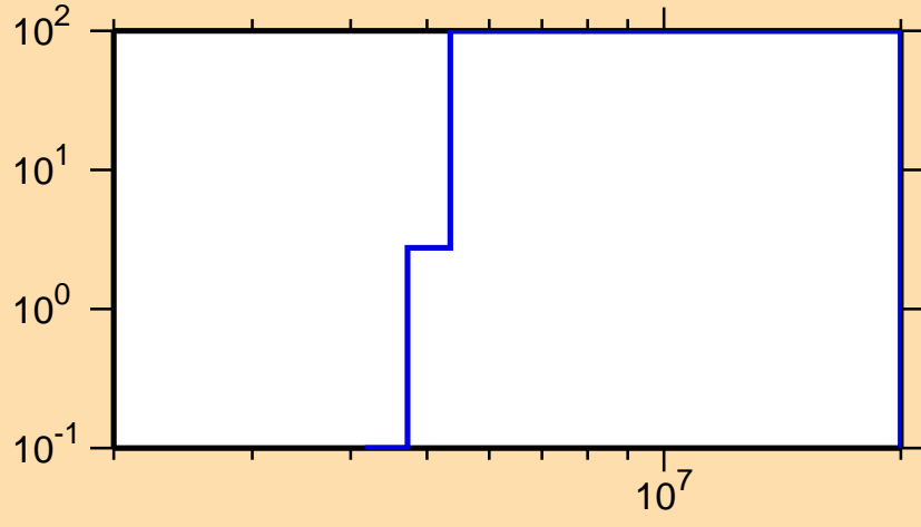
\Delta\sigma/\sigma vs. E for ^{237}\text{Pa}(n,p)
