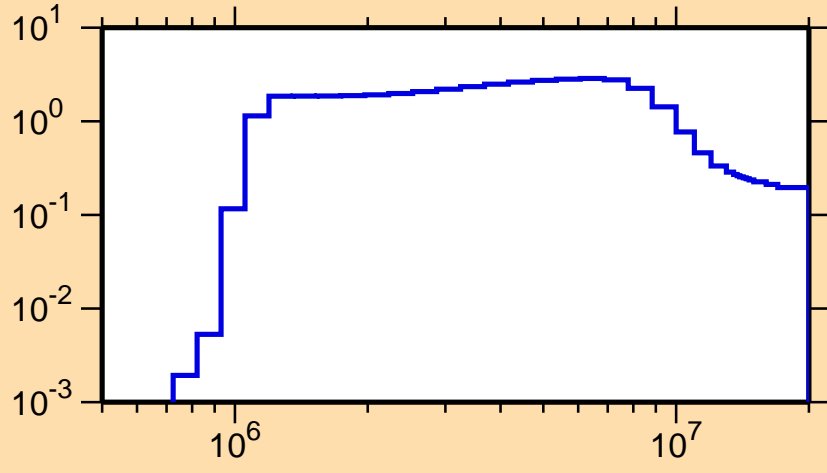
\sigma vs. E for ^{237}\text{Pa}(n,n\text{cont.})
