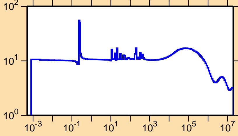
\sigma vs. E for ^{237}\text{Pa}(n,\text{el.})
