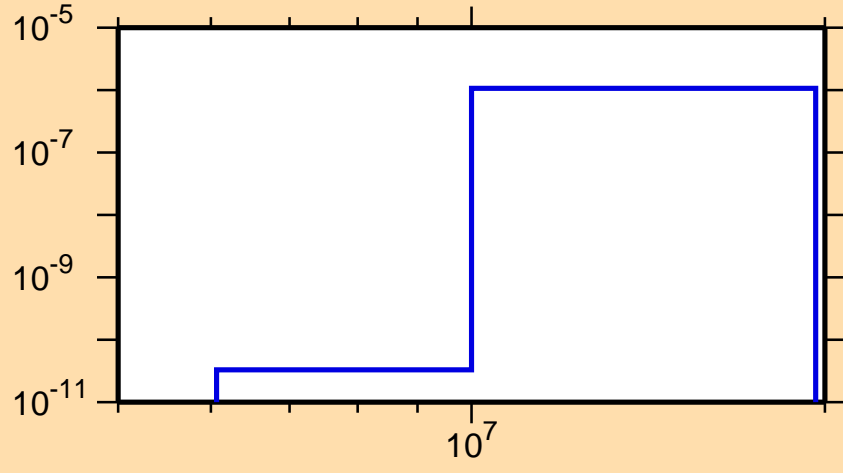
\sigma vs. E for ^{237}\text{Pa}(n,n\alpha)
