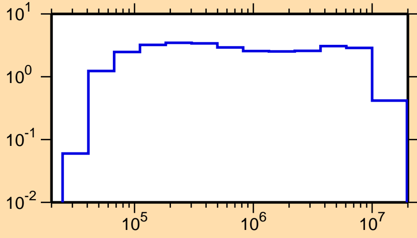
\sigma vs. E for ^{237}\text{Pa}(n,\text{inel.})
