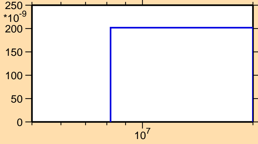
\sigma vs. E for ^{237}\text{Pa}(n,nt)
