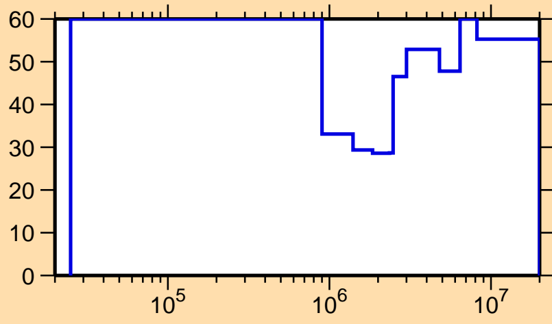
\Delta\sigma/\sigma vs. E for ^{237}\text{Pa}(n,\text{inel.})
