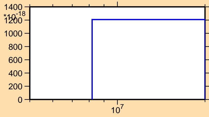
\sigma vs. E for ^{237}\text{Pa}(n,\text{He3})
