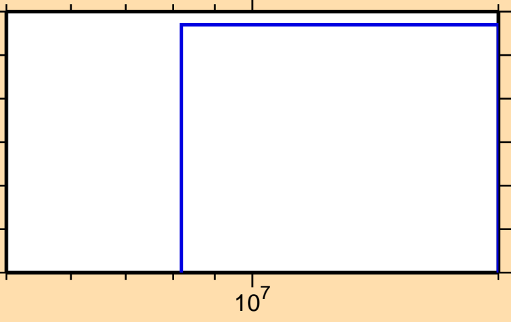
\sigma vs. E for ^{237}\text{Pa}(n,3n\alpha)
