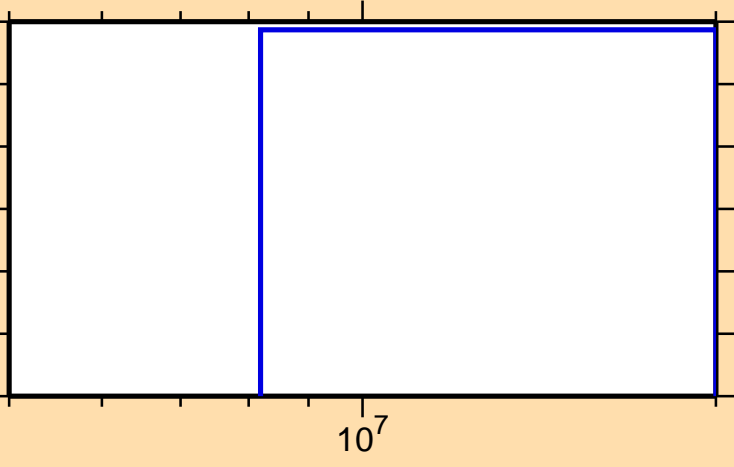
\sigma vs. E for ^{237}\text{Pa}(n,\text{nd})
