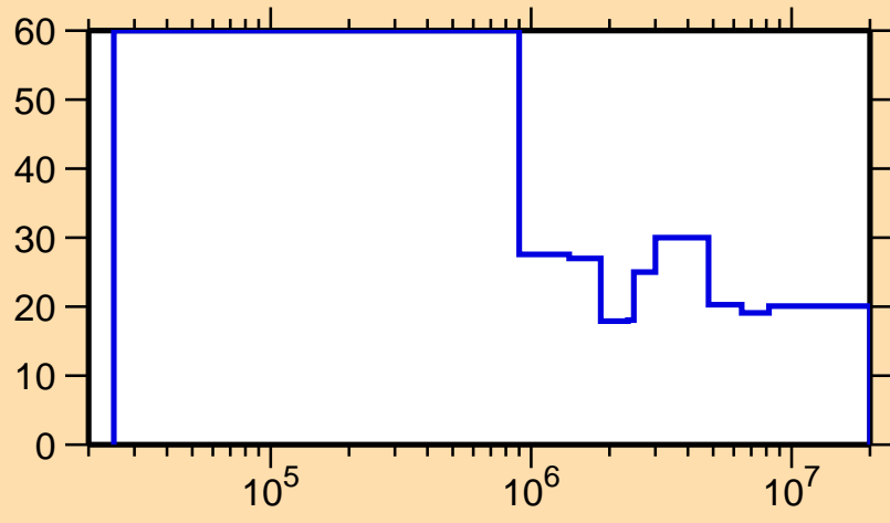
\Delta\sigma/\sigma vs. E for ^{237}\text{Pa}(n,\text{nonel.})
