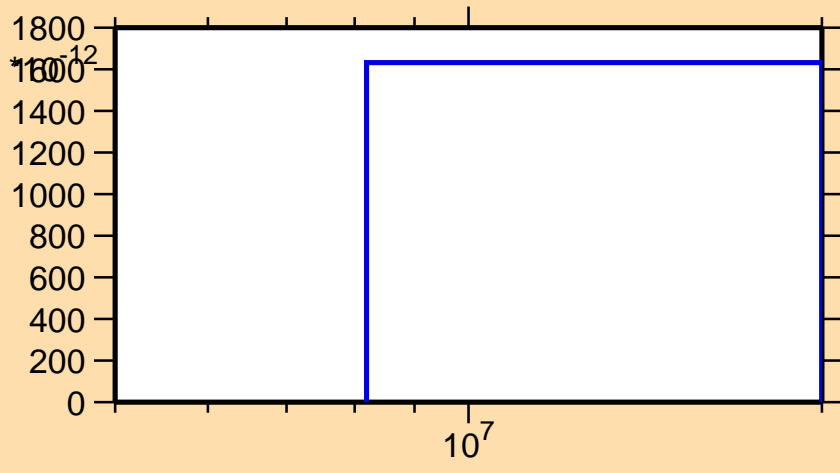
\sigma vs. E for ^{237}\text{Pa}(n,2n\alpha)
