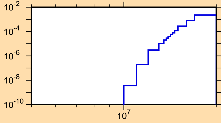
\sigma vs. E for ^{238}\text{Pa}(n,np)
