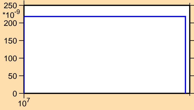
\sigma vs. E for ^{238}\text{Pa}(n,2np)
