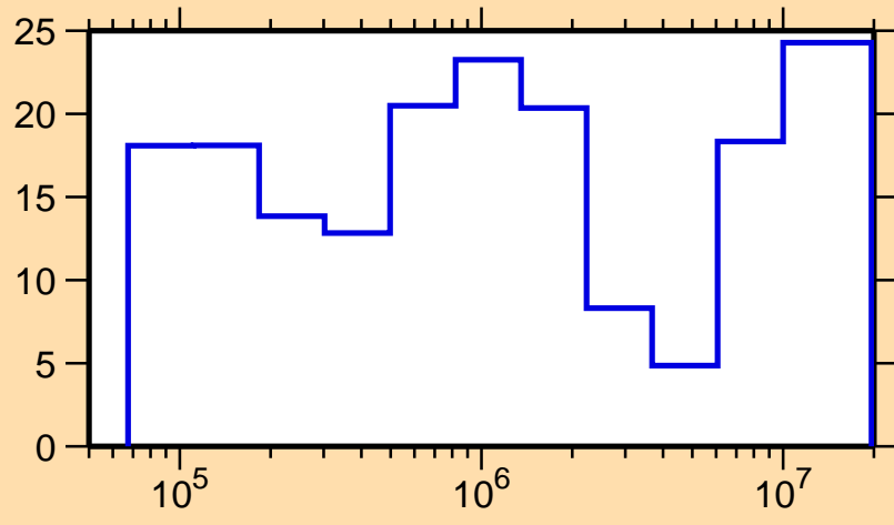
\Delta\sigma/\sigma vs. E for ^{238}\text{Pa}(n, tot.)
