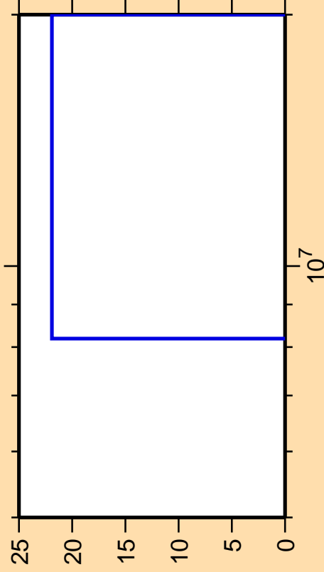
\Delta\sigma/\sigma vs. E for ^{238}\text{Pa}(n,nd)
