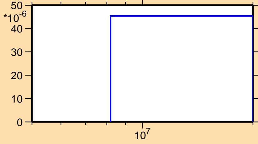
\sigma vs. E for ^{238}\text{Pa}(n,d)
