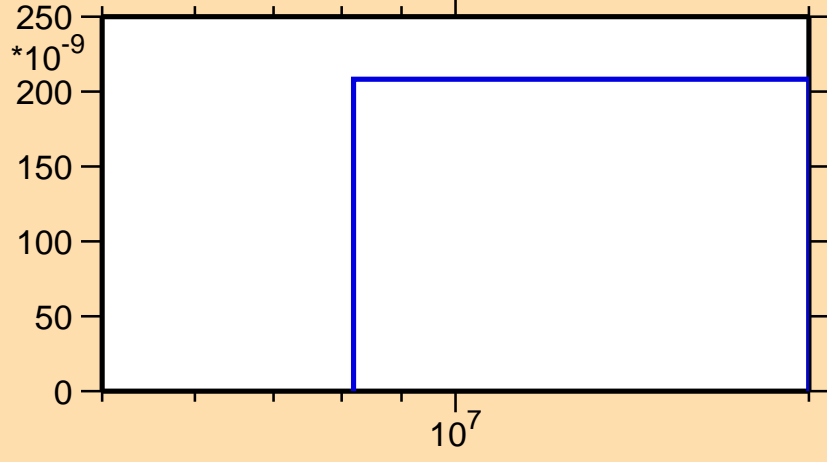
\sigma vs. E for ^{238}\text{Pa}(n,nd)
