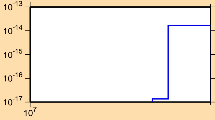
\sigma vs. E for ^{239}\text{Pa} (mt 11)
