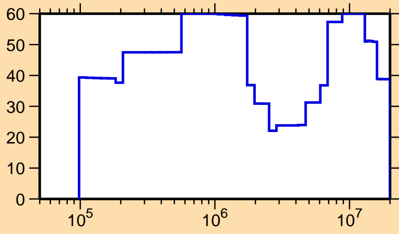
\Delta\sigma/\sigma vs. E for ^{239}\text{Pa}(n, el.)
