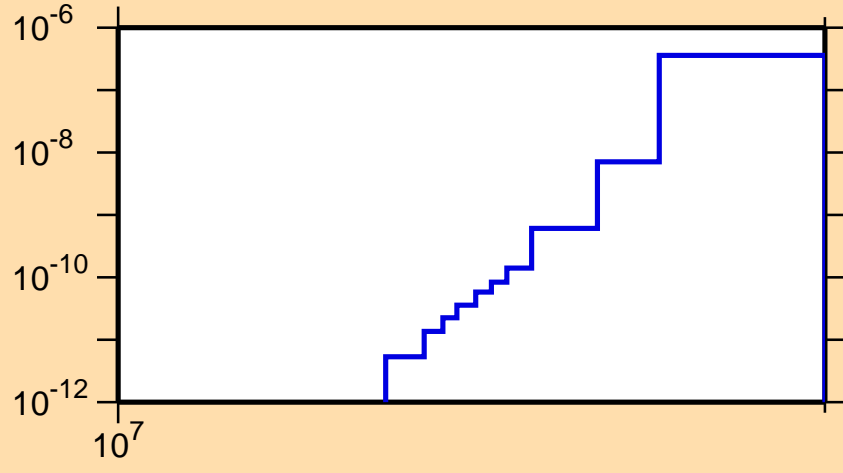
\sigma vs. E for ^{239}\text{Pa}(n,2n\alpha)
