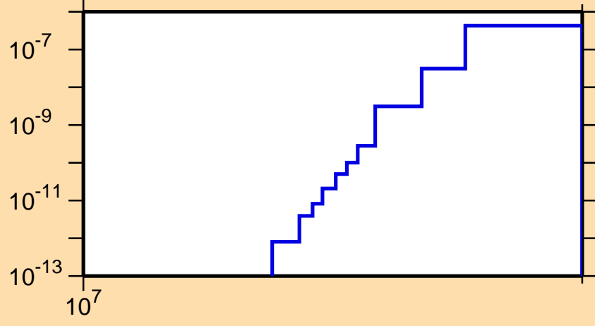
\sigma vs. E for ^{239}\text{Pa}(n,nt)
