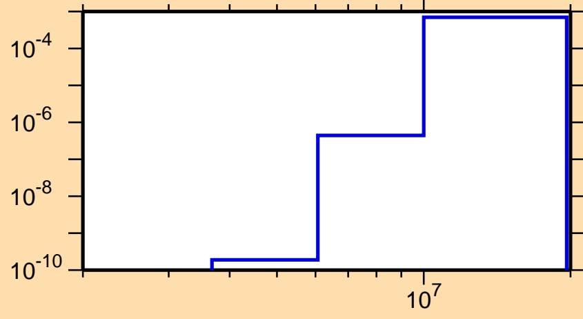
\sigma vs. E for ^{239}\text{Pa}(n,\alpha)
