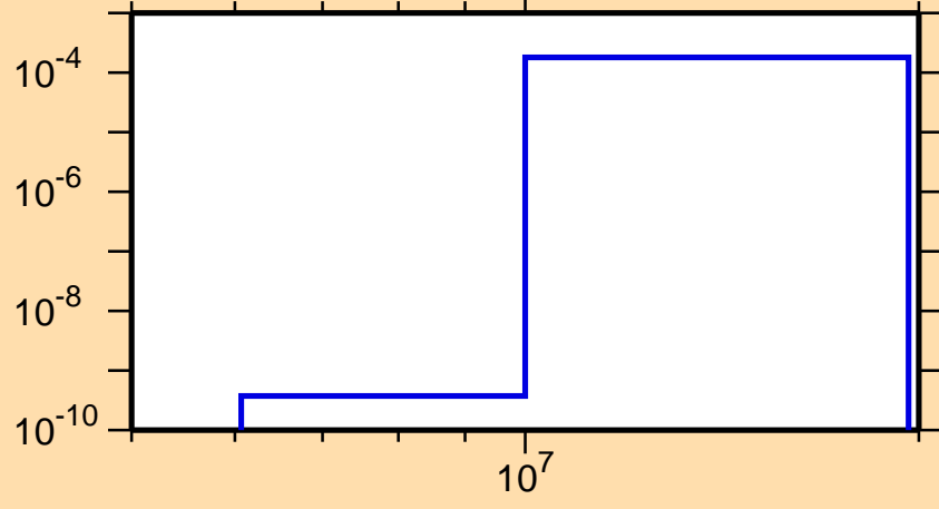
\sigma vs. E for ^{239}\text{Pa}(n,n\alpha)
