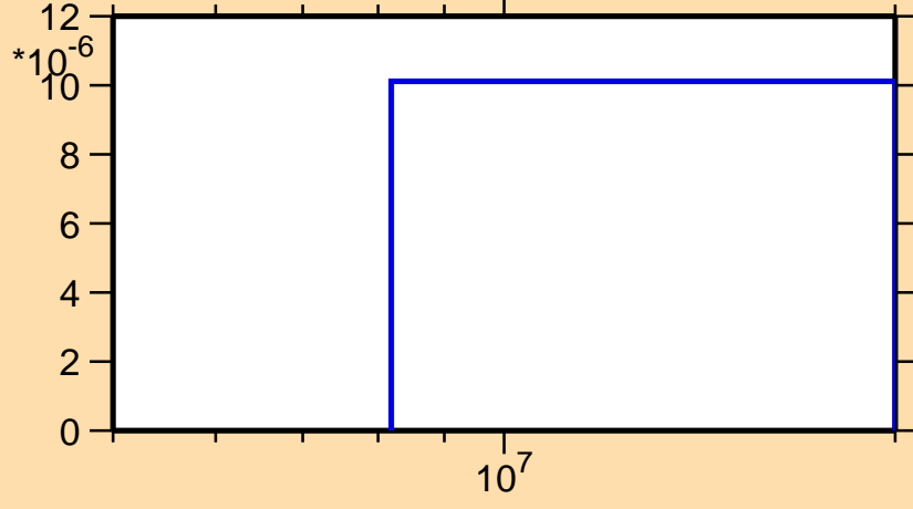
\sigma vs. E for ^{239}\text{Pa}(n,t)
