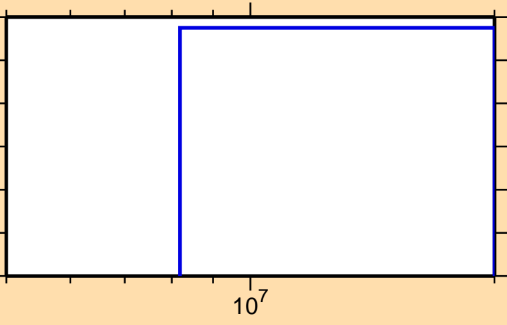
\sigma vs. E for ^{239}\text{Pa}(n,\text{nd})
