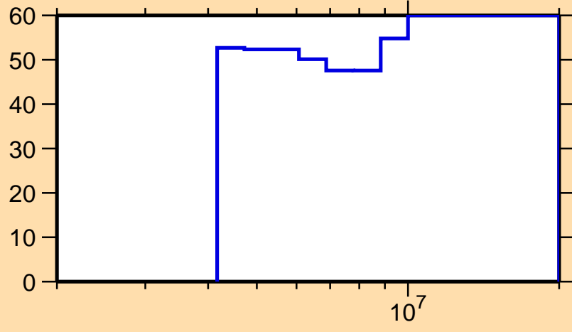
\Delta\sigma/\sigma vs. E for ^{240}\text{Pa}(n,2n)
