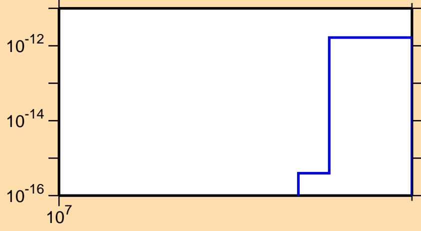
\sigma vs. E for ^{240}\text{Pa} (mt 11)
