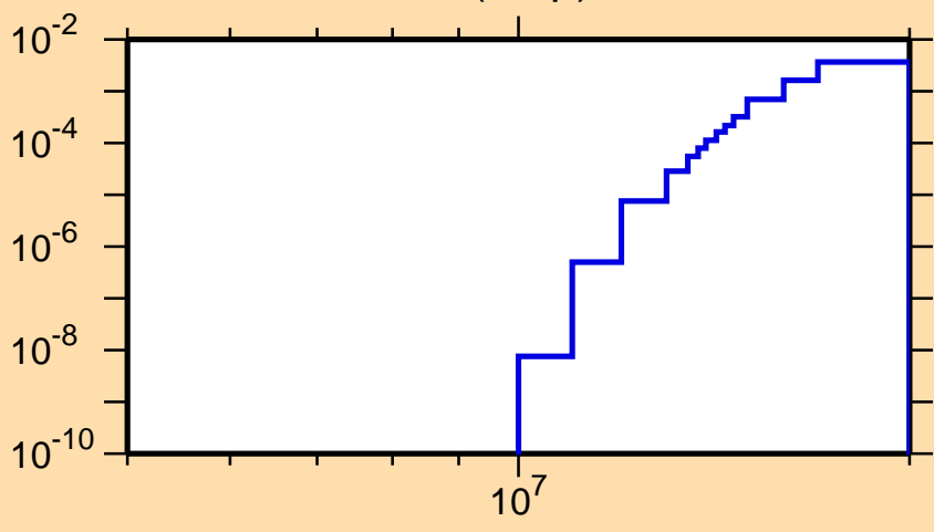
\sigma vs. E for ^{240}\text{Pa}(n,np)
