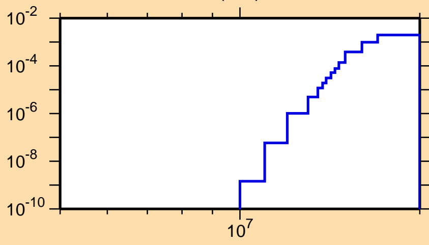
\sigma vs. E for ^{240}\text{Pa}(n,d)
