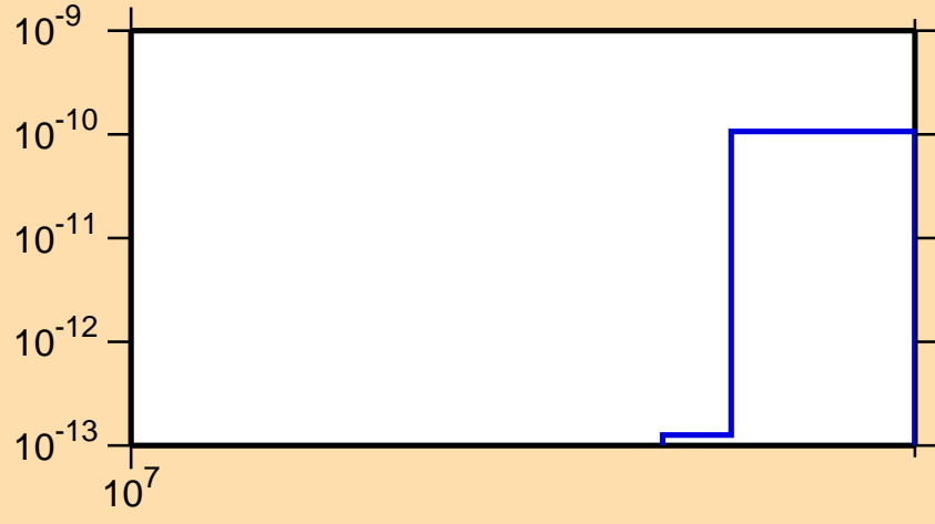
\sigma vs. E for ^{240}\text{Pa}(n,3n\alpha)
