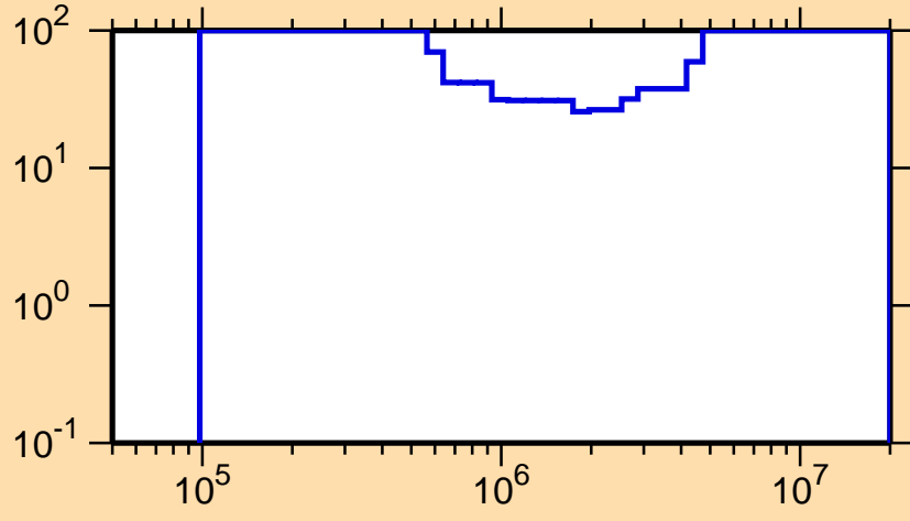
\Delta\sigma/\sigma vs. E for ^{240}\text{Pa}(n,\text{inel.})
