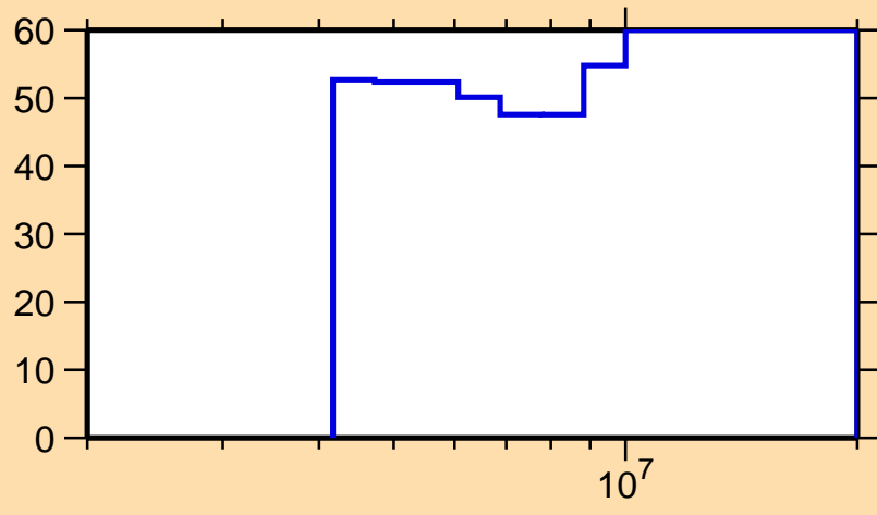
\Delta\sigma/\sigma vs. E for ^{240}\text{Pa}(n,2n)
