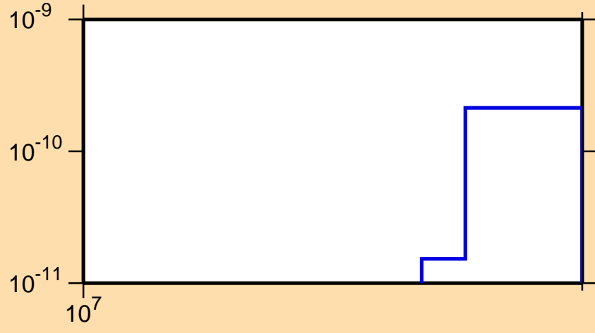
\sigma vs. E for ^{240}\text{Pa}(n,\text{He}3)
