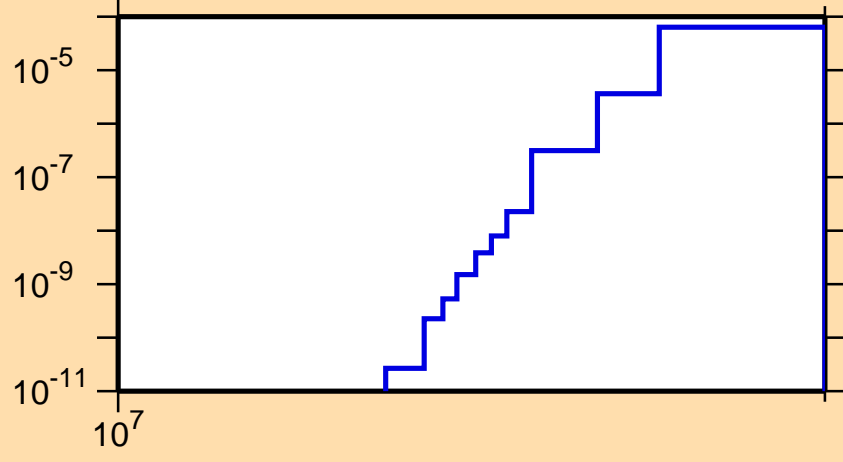
\sigma vs. E for ^{240}\text{Pa}(n,\text{nd})
