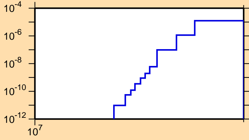
\sigma vs. E for ^{240}\text{Pa}(n,nt)
