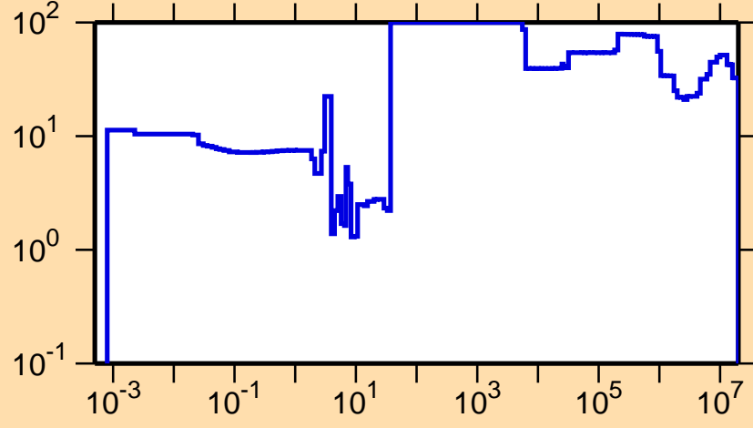
\Delta\sigma/\sigma vs. E for ^{240}\text{Pa}(n,\text{tot.})
