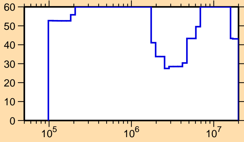
\Delta\sigma/\sigma vs. E for ^{240}\text{Pa}(n,\text{el.})
