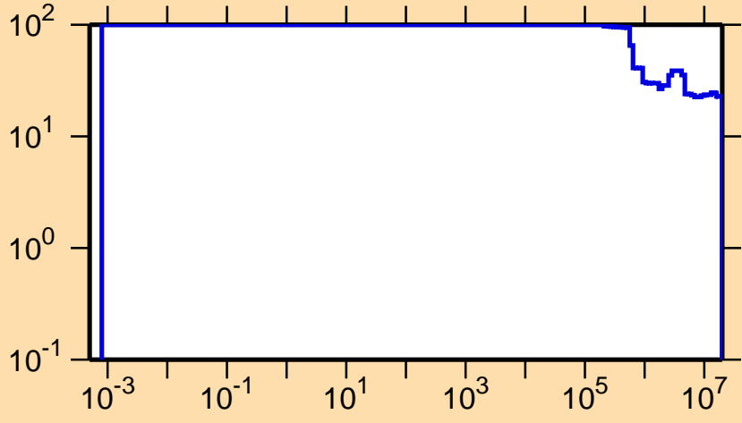
\Delta\sigma/\sigma vs. E for ^{240}\text{Pa}(n,\text{nonel.})
