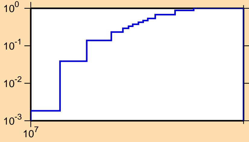
\sigma vs. E for ^{240}\text{Pa}(n,3n)
