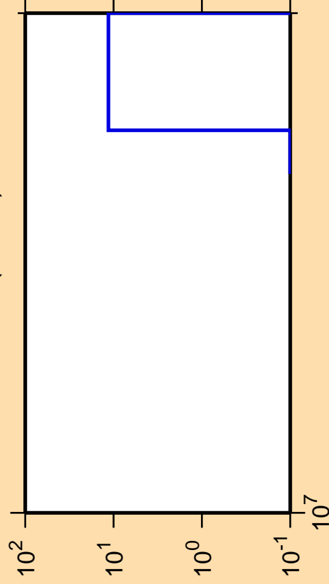
\Delta\sigma/\sigma vs. E for ^{240}\text{Pa} (mt 11)
