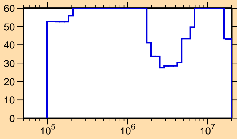
\Delta\sigma/\sigma vs. E for ^{240}\text{Pa}(n,\text{el.})
