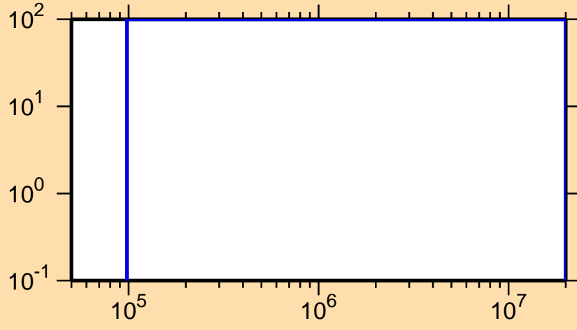
\Delta\sigma/\sigma vs. E for ^{240}\text{Pa}(n,n_1)
