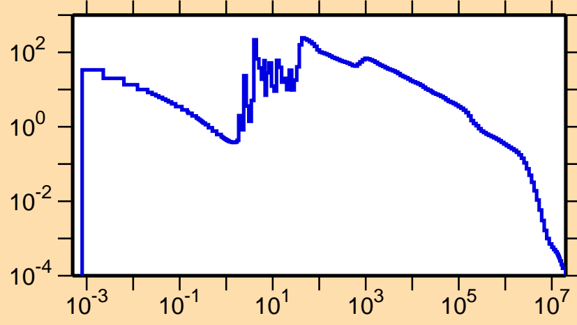
\sigma vs. E for ^{240}\text{Pa}(n,\gamma)
