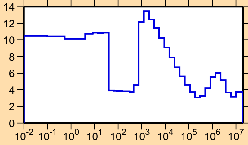
\sigma vs. E for ^{240}\text{Pa}(n,\text{el.})
