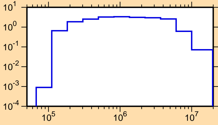
\sigma vs. E for ^{240}\text{Pa}(n,\text{inel.})
