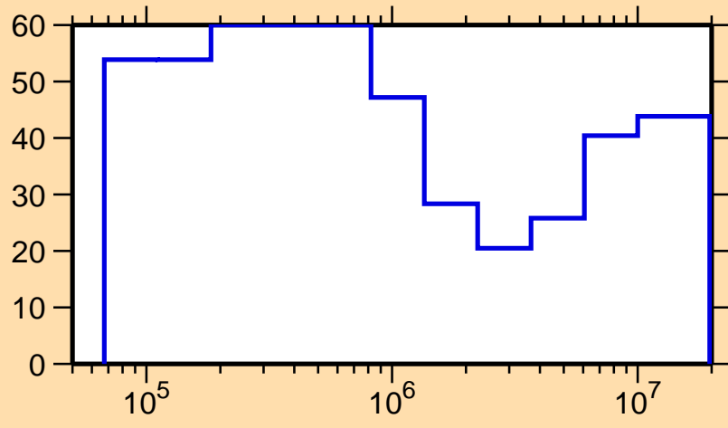
\Delta\sigma/\sigma vs. E for ^{240}\text{Pa}(n,\text{tot.})
