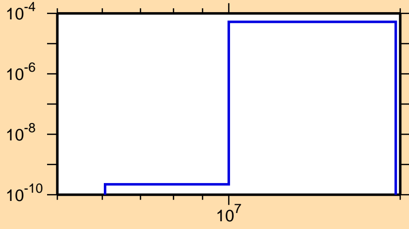
\sigma vs. E for ^{240}\text{Pa}(n,n\alpha)
