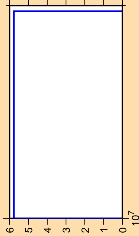
\Delta\sigma/\sigma vs. E for ^{240}\text{Pa}(n,3n\alpha)
