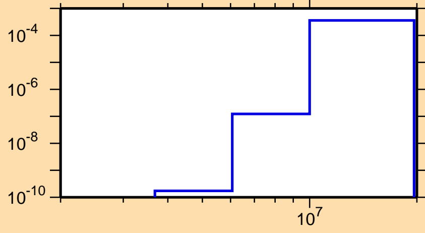
\sigma vs. E for ^{240}\text{Pa}(n,\alpha)
