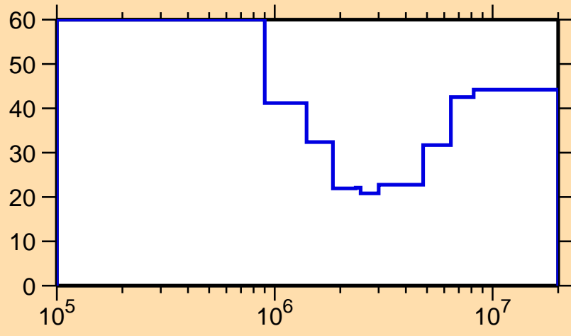
\Delta\sigma/\sigma vs. E for ^{240}\text{Pa}(n, tot.)
