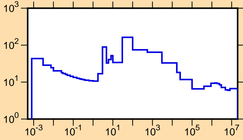
\sigma vs. E for ^{240}\text{Pa}(n,\text{tot.})
