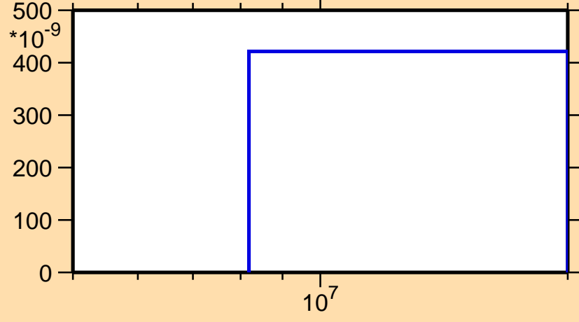
\sigma vs. E for ^{240}\text{Pa}(n,2np)
