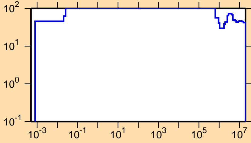
\Delta\sigma/\sigma vs. E for ^{241}\text{Pa}(n,\text{nonel.})
