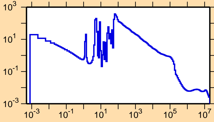
\sigma vs. E for ^{241}\text{Pa}(n,\gamma)
