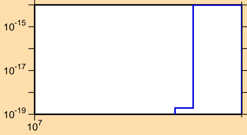
\sigma vs. E for ^{241}\text{Pa} (mt 11)
