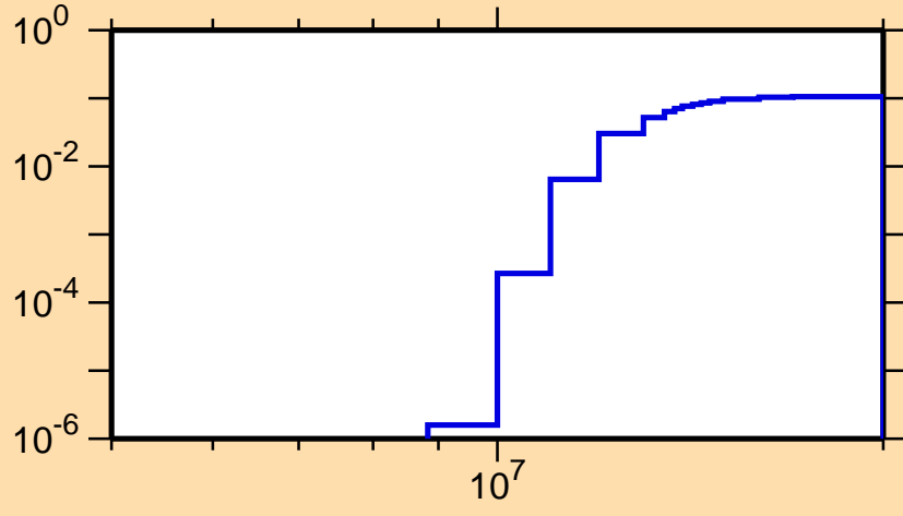
\sigma vs. E for ^{241}\text{Pa}(n,np)
