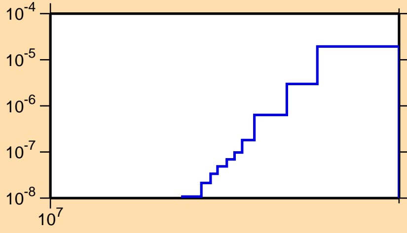
\sigma vs. E for ^{241}\text{Pa}(n,2n\alpha)
