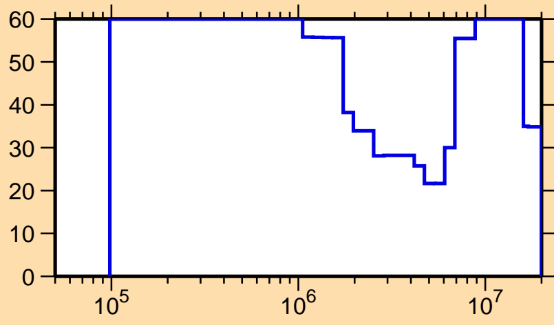
\Delta\sigma/\sigma vs. E for ^{241}\text{Pa}(n,\text{el.})
