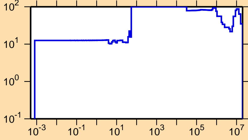
\Delta\sigma/\sigma vs. E for ^{241}\text{Pa}(n,\text{el.})
