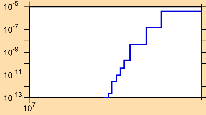
\sigma vs. E for ^{241}\text{Pa}(n,\text{nd})
