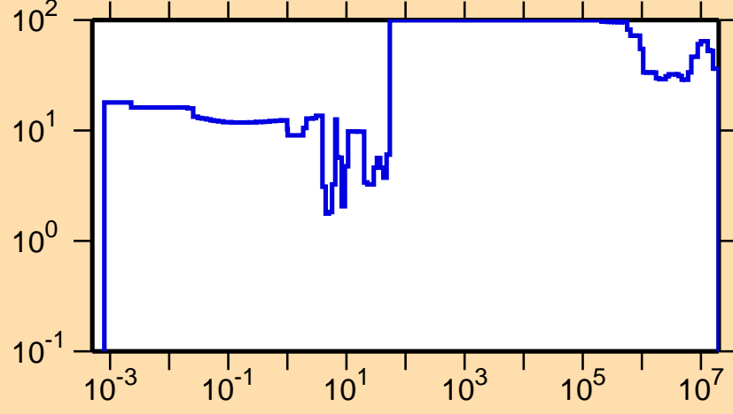
\Delta\sigma/\sigma vs. E for ^{241}\text{Pa}(n,\text{tot.})
