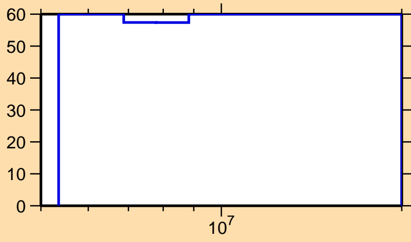
\Delta\sigma/\sigma vs. E for ^{241}\text{Pa}(n,2n)
