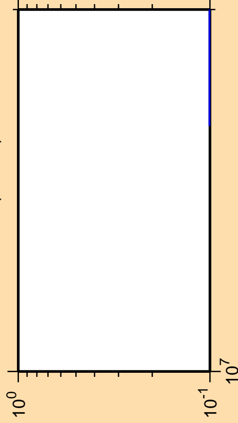
\Delta\sigma/\sigma vs. E for ^{241}\text{Pa} (mt 11)
