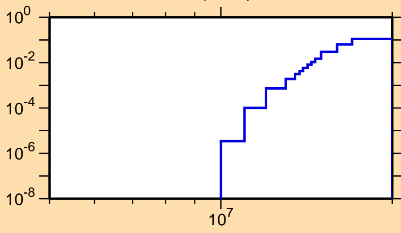
\sigma vs. E for ^{241}\text{Pa}(n,3n)
