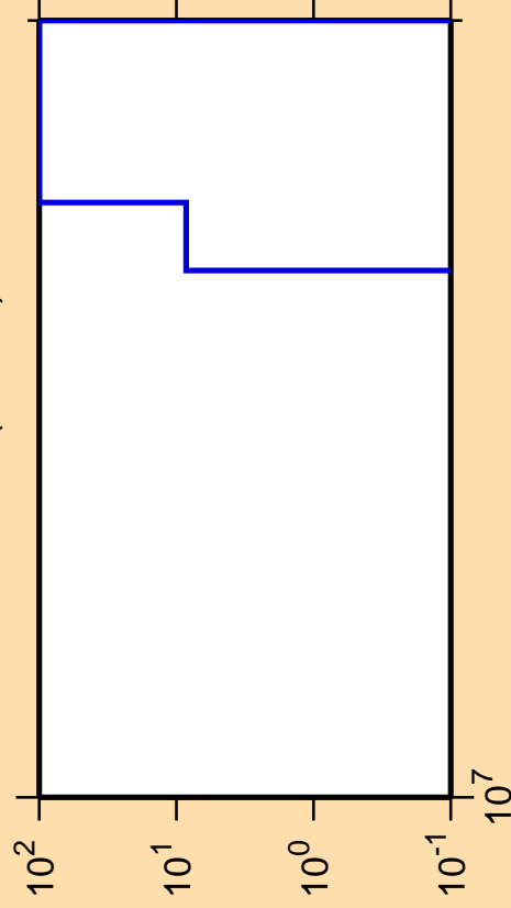
\Delta\sigma/\sigma vs. E for ^{241}\text{Pa}(n,3n\alpha)
