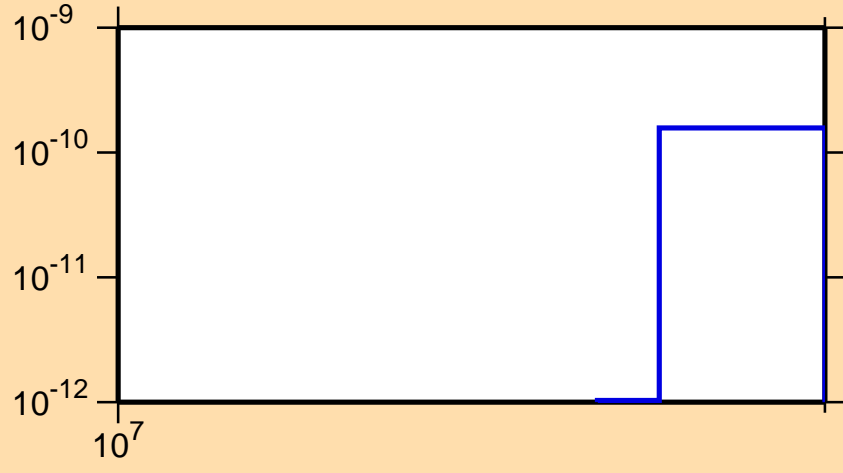
\sigma vs. E for ^{241}\text{Pa}(n,3n\alpha)
