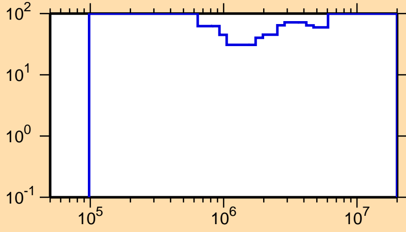
\Delta\sigma/\sigma vs. E for ^{241}\text{Pa}(n,\text{inel.})
