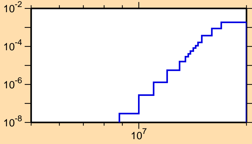
\sigma vs. E for ^{241}\text{Pa}(n,d)
