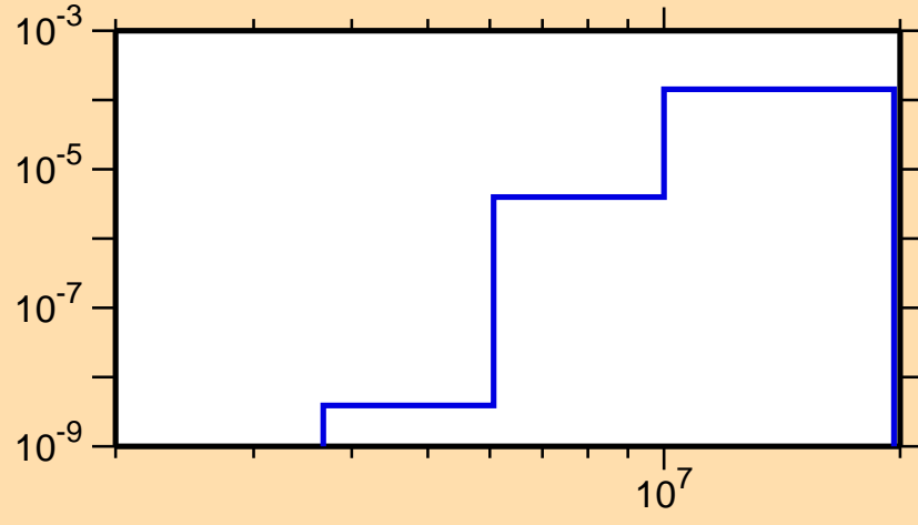
\sigma vs. E for ^{241}\text{Pa}(n,\alpha)
