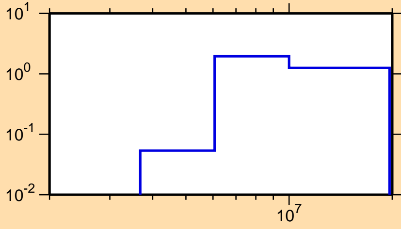
\sigma vs. E for ^{241}\text{Pa}(n,2n)
