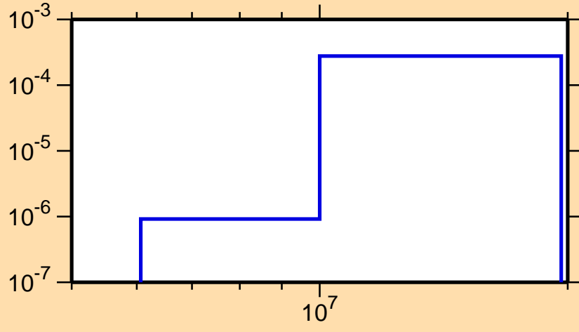
\sigma vs. E for ^{241}\text{Pa}(n,n\alpha)
