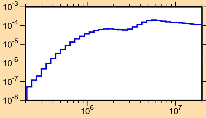
\sigma vs. E for ^{185}\text{Pb}(n,n_1)
