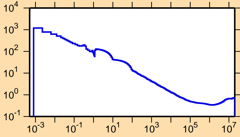
\sigma vs. E for ^{185}\text{Pb}(n,\text{nonel.})
