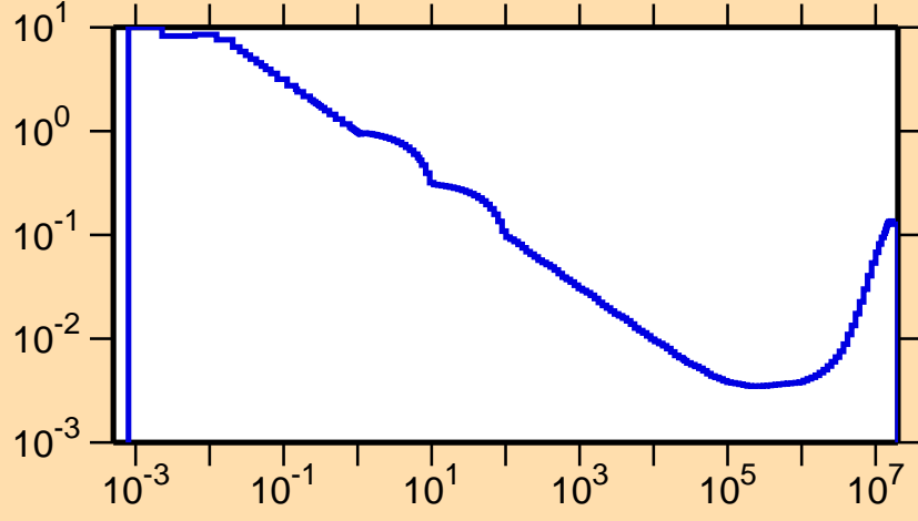
\sigma vs. E for ^{185}\text{Pb}(n,\alpha)
