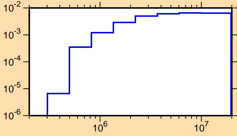
\sigma vs. E for ^{185}\text{Pb}(n,n_4)
