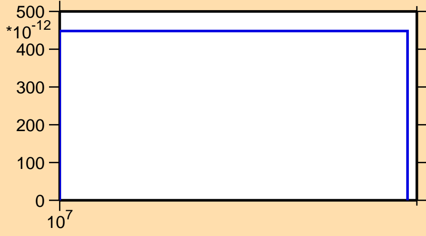
\sigma vs. E for ^{185}\text{Pb} (mt 34)
