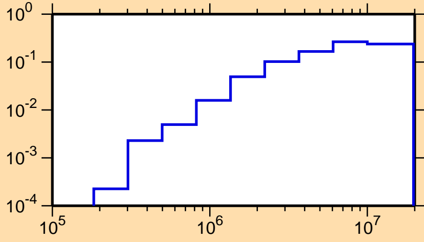
\sigma vs. E for ^{185}\text{Pb}(n,\text{inel.})
