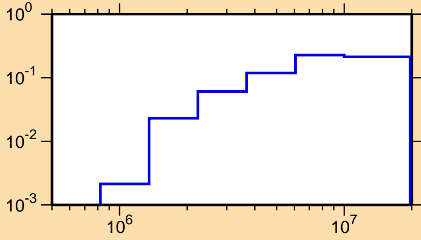
\sigma vs. E for ^{185}\text{Pb}(n,n\text{cont.})
