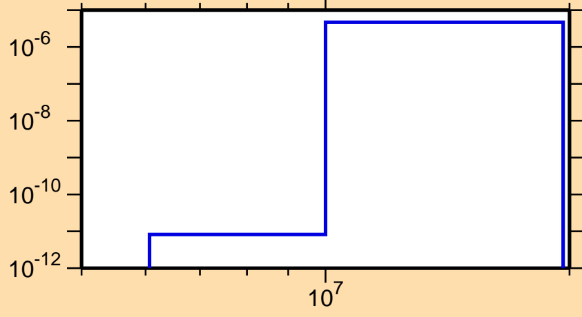
\sigma vs. E for ^{185}\text{Pb}(n,pd)
