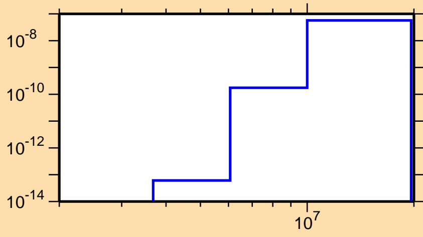
\sigma vs. E for ^{185}\text{Pb}(\text{mt117})
