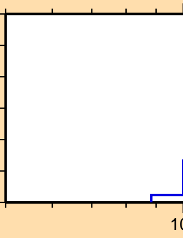
\sigma vs. E for ^{186}\text{Pb}(\text{mt117})
