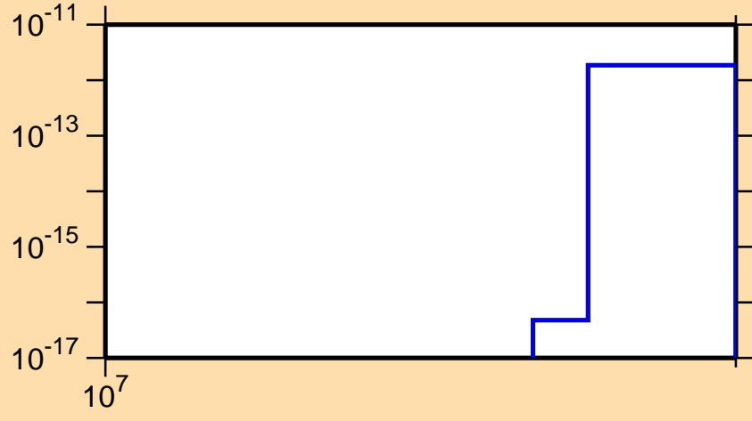
\sigma vs. E for ^{186}\text{Pb}(n,nt)
