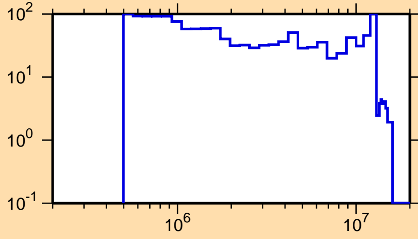
\Delta\sigma/\sigma vs. E for ^{186}\text{Pb}(n,n_1)
