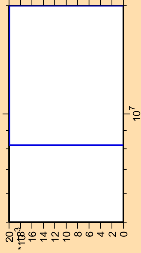
\Delta\sigma/\sigma vs. E for ^{186}\text{Pb}(n,3n)
