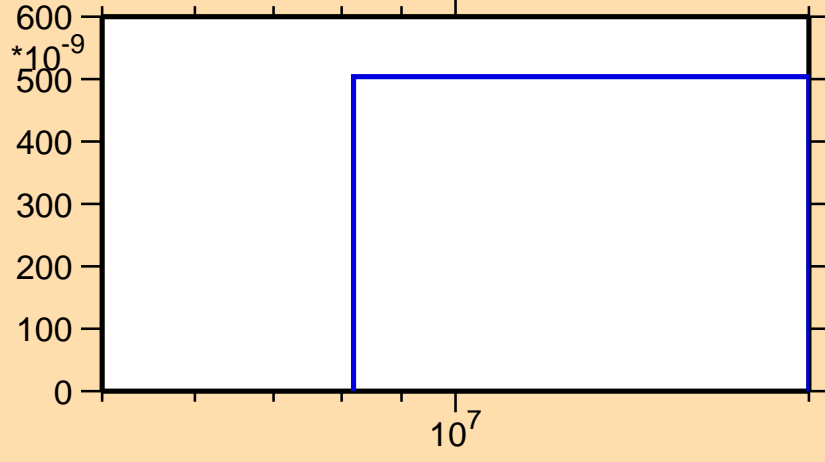
\sigma vs. E for ^{186}\text{Pb}(\text{mt } 45)
