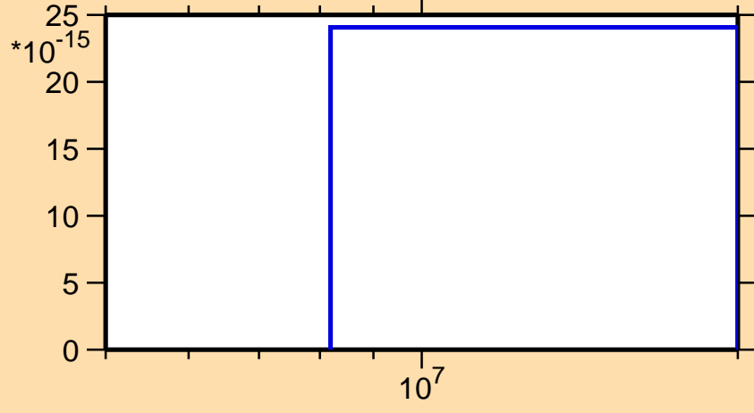
\sigma vs. E for ^{186}\text{Pb}(n,3n)
