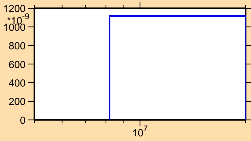
\sigma vs. E for ^{186}\text{Pb}(n,\text{pd})
