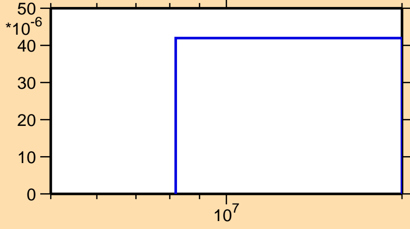
\sigma vs. E for ^{186}\text{Pb}(n,t)
