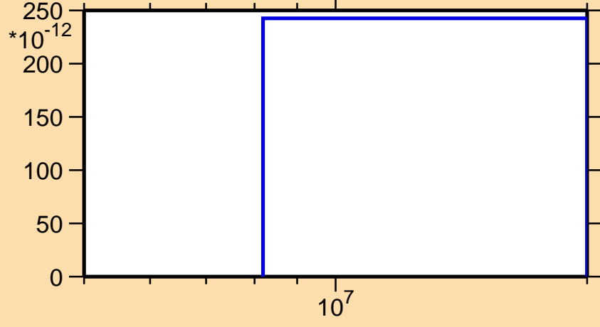
\sigma vs. E for ^{186}\text{Pb}(n,nd)
