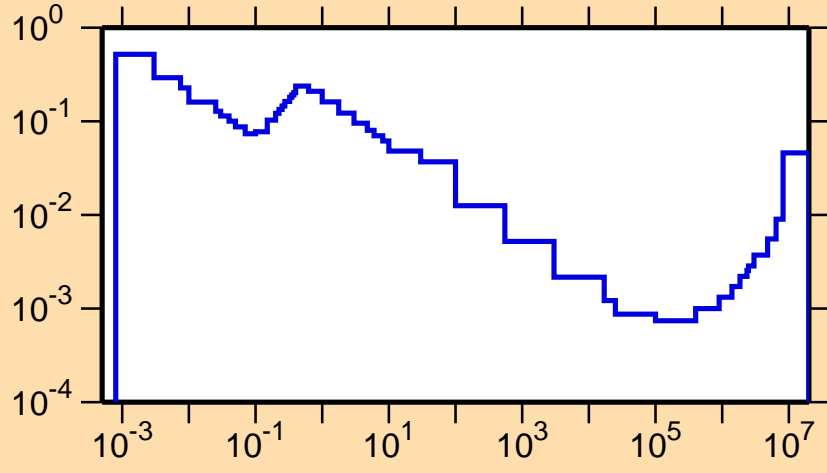
\sigma vs. E for ^{186}\text{Pb}(n,\alpha)
