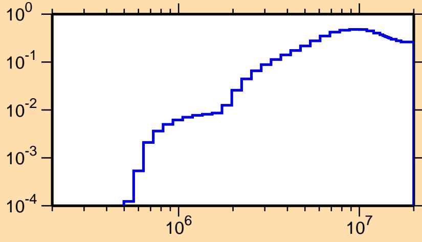
\sigma vs. E for ^{187}\text{Pb}(n,n\text{cont.})
