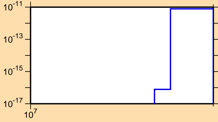
\sigma vs. E for ^{188}\text{Pb}(n,nt)
