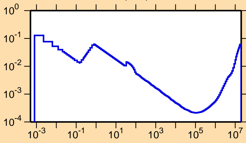
\sigma vs. E for ^{188}\text{Pb}(n,\alpha)
