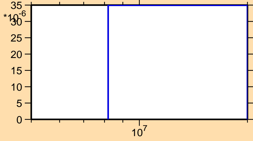
\sigma vs. E for ^{188}\text{Pb}(n,t)
