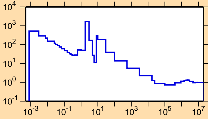
\sigma vs. E for ^{188}\text{Pb}(n,\text{nonel.})
