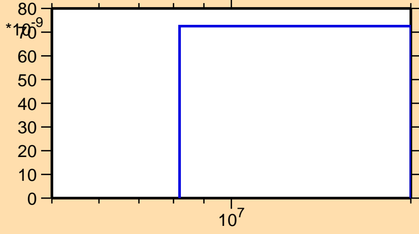
\sigma vs. E for ^{188}\text{Pb}(n,2n\alpha)
