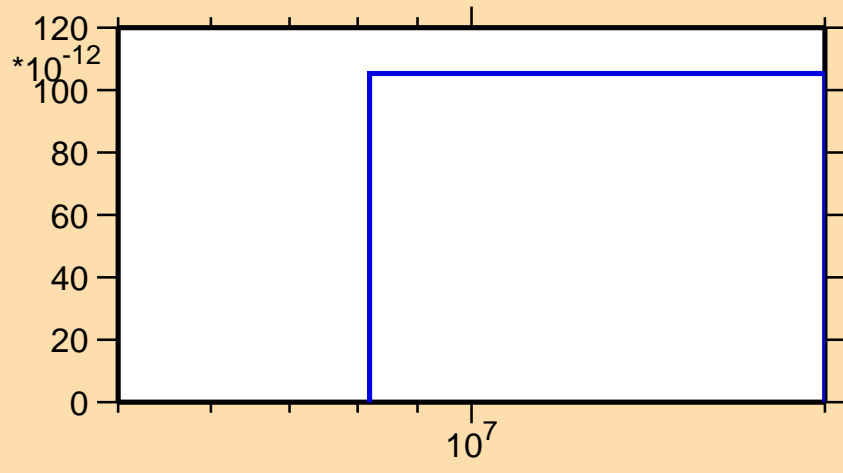
\sigma vs. E for ^{188}\text{Pb}(n,3n)
