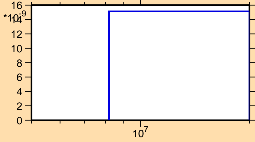
\sigma vs. E for ^{188}\text{Pb}(n,2np)
