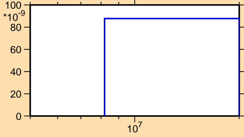
\sigma vs. E for ^{188}\text{Pb}(n,\text{pd})
