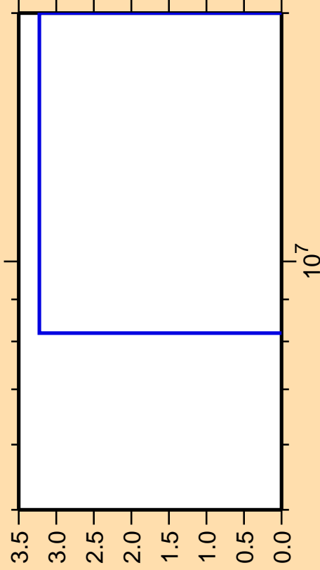
\Delta\sigma/\sigma vs. E for ^{188}\text{Pb}(\text{mt } 34)
