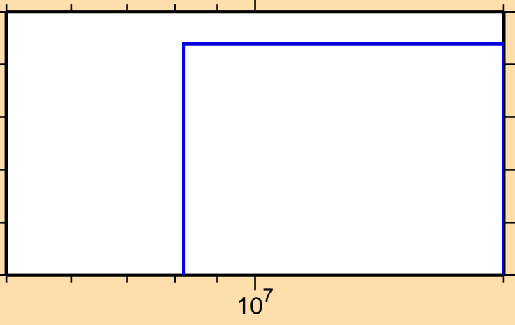
\sigma vs. E for ^{188}\text{Pb}(\text{mt } 34)
