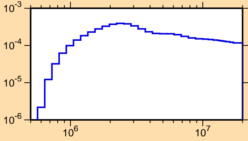
\sigma vs. E for ^{189}\text{Pb}(n,n_3)
