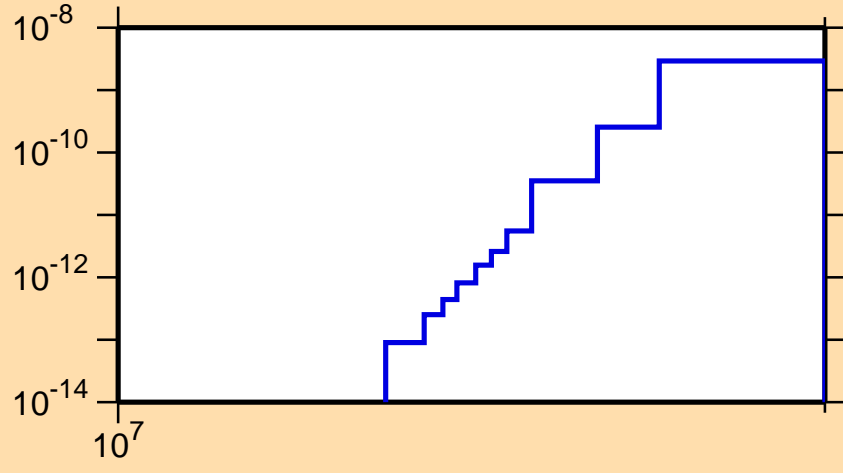
\sigma vs. E for ^{189}\text{Pb}(\text{mt } 34)
