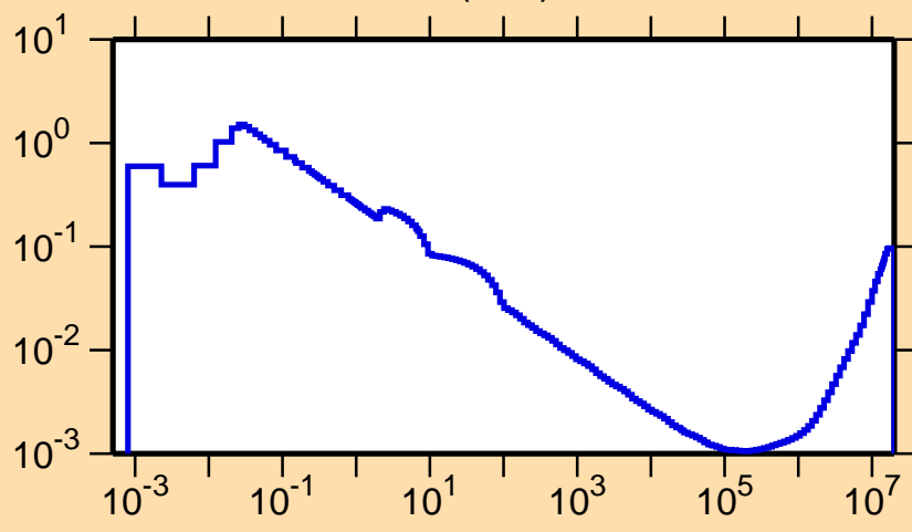
\sigma vs. E for ^{189}\text{Pb}(n,\alpha)
