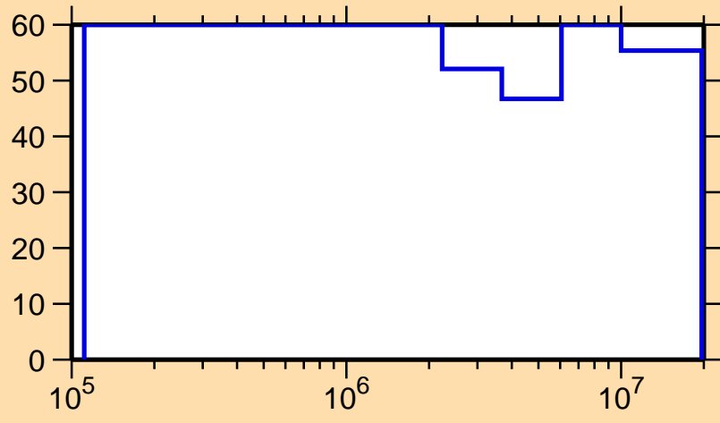
\Delta\sigma/\sigma vs. E for ^{189}\text{Pb}(n,n_1)
