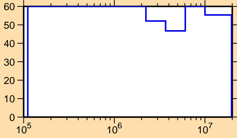
\Delta\sigma/\sigma vs. E for ^{189}\text{Pb}(n,n_1)
