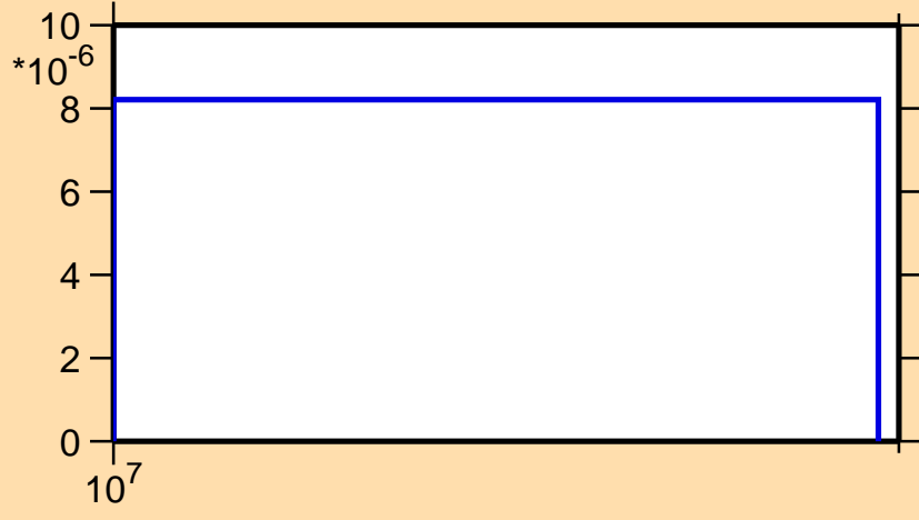
\sigma vs. E for ^{189}\text{Pb}(n,2np)
