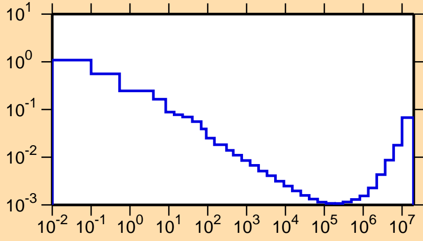
\sigma vs. E for ^{189}\text{Pb}(n,\alpha)
