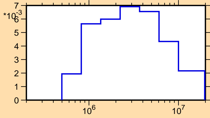
\sigma vs. E for ^{189}\text{Pb}(n,n_4)
