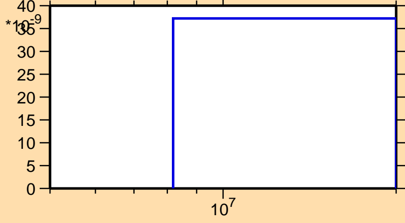
\sigma vs. E for ^{189}\text{Pb}(n,pd)
