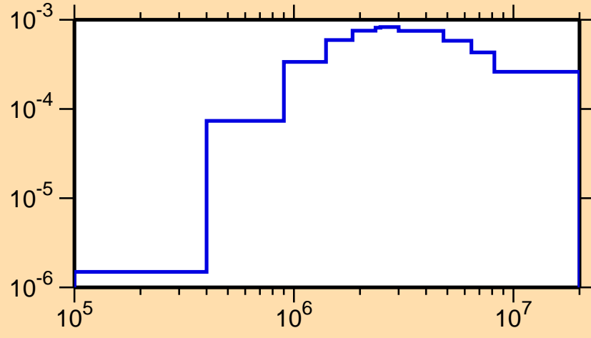
\sigma vs. E for ^{189}\text{Pb}(n,n_1)
