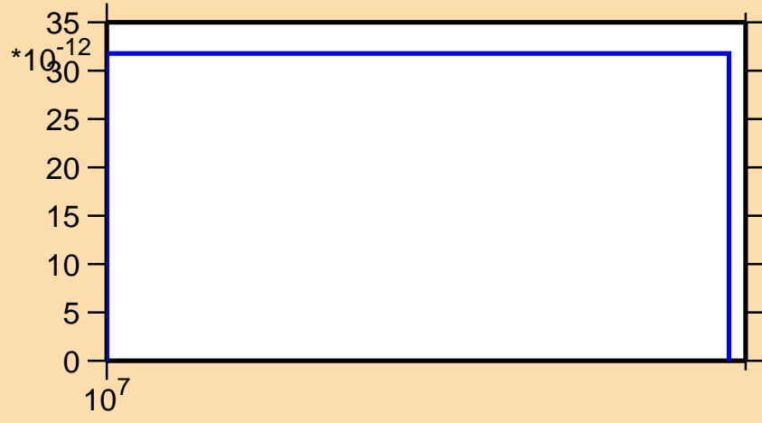
\sigma vs. E for ^{189}\text{Pb} (mt 34)
