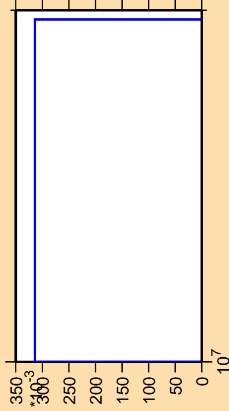
\Delta\sigma/\sigma vs. E for ^{189}\text{Pb}(n,nt)
