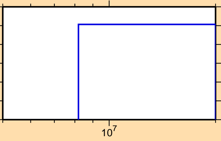
\sigma vs. E for ^{189}\text{Pb}(\text{mt } 45)
