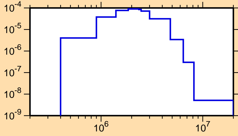
\sigma vs. E for ^{189}\text{Pb}(n,n_2)
