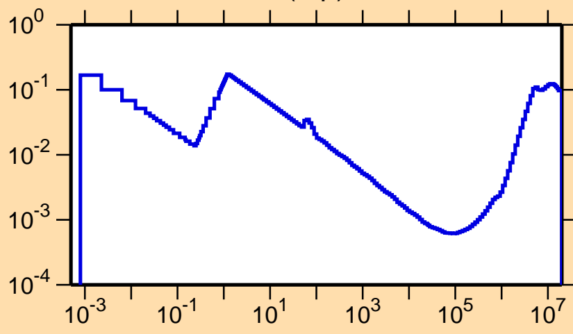
\sigma vs. E for ^{190}\text{Pb}(n,p)
