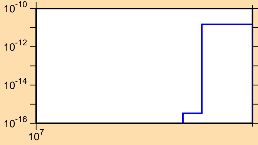
\sigma vs. E for ^{190}\text{Pb}(n,nt)
