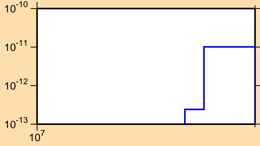
\sigma vs. E for ^{190}\text{Pb}(\text{mt } 34)
