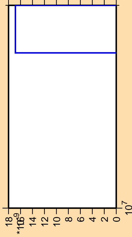
\Delta\sigma/\sigma vs. E for ^{190}\text{Pb} (mt 11)
