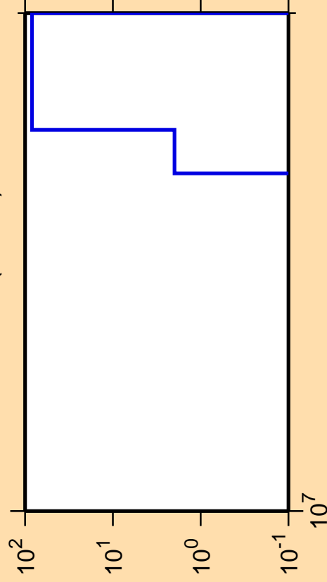
\Delta\sigma/\sigma vs. E for ^{190}\text{Pb}(\text{mt } 34)
