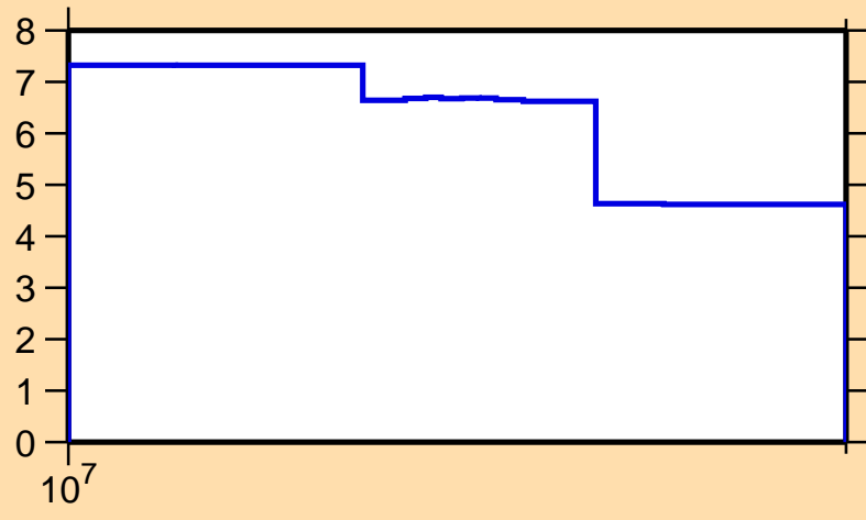
\Delta\sigma/\sigma vs. E for ^{190}\text{Pb}(n,\text{tot.})
