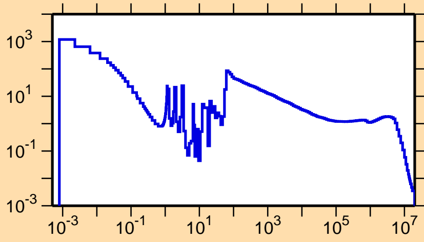
\sigma vs. E for ^{190}\text{Pb}(n,\gamma)
