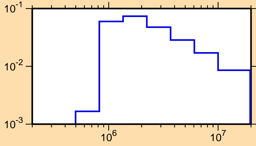
\sigma vs. E for ^{190}\text{Pb}(n,n_2)
