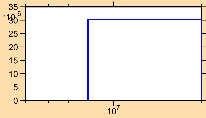
\sigma vs. E for ^{190}\text{Pb}(n,t)
