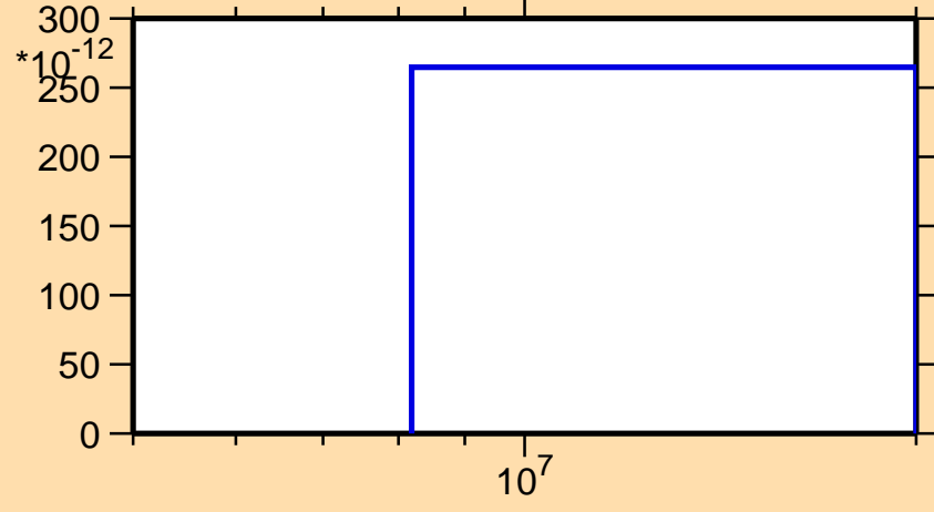
\sigma vs. E for ^{190}\text{Pb}(\text{mt117})
