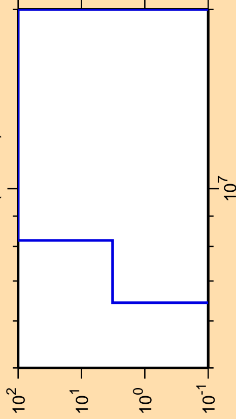
\Delta\sigma/\sigma vs. E for ^{190}\text{Pb}(n,\text{He3})
