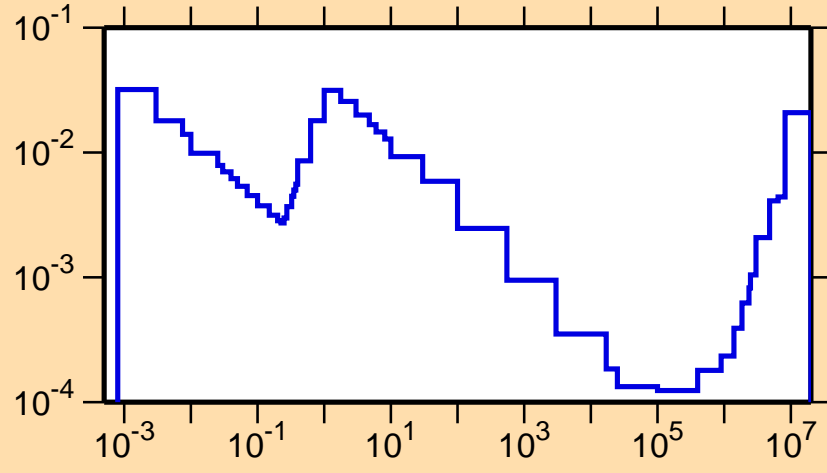
\sigma vs. E for ^{190}\text{Pb}(n,\alpha)
