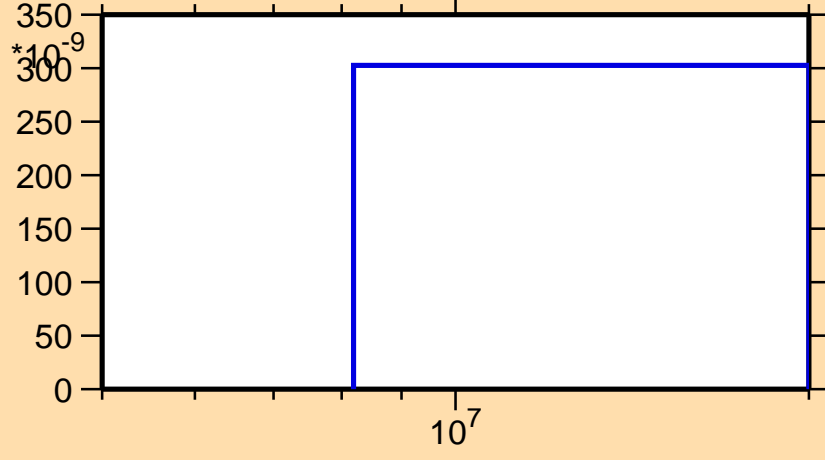
\sigma vs. E for ^{190}\text{Pb}(n,2n\alpha)
