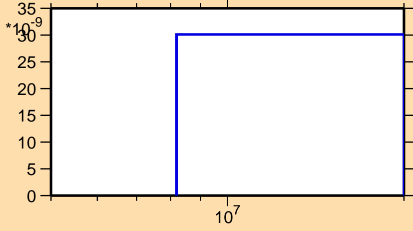
\sigma vs. E for ^{190}\text{Pb}(n,2np)
