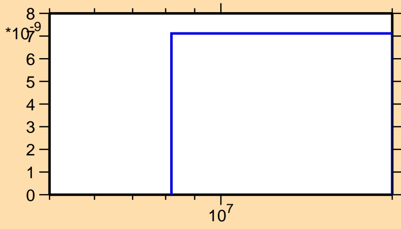
\sigma vs. E for ^{190}\text{Pb}(n,\text{pd})
