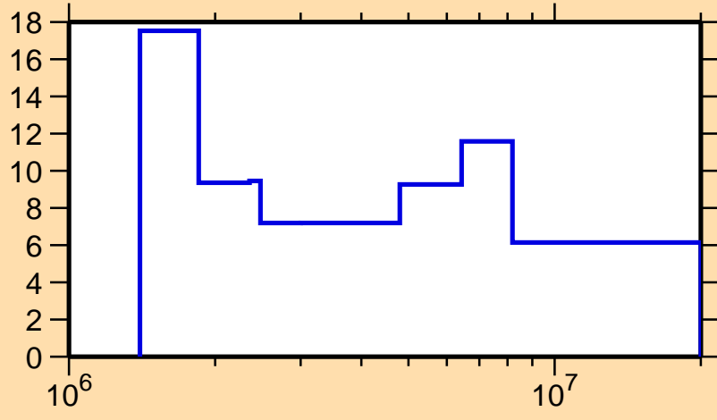
\Delta\sigma/\sigma vs. E for ^{190}\text{Pb}(n,\text{tot.})
