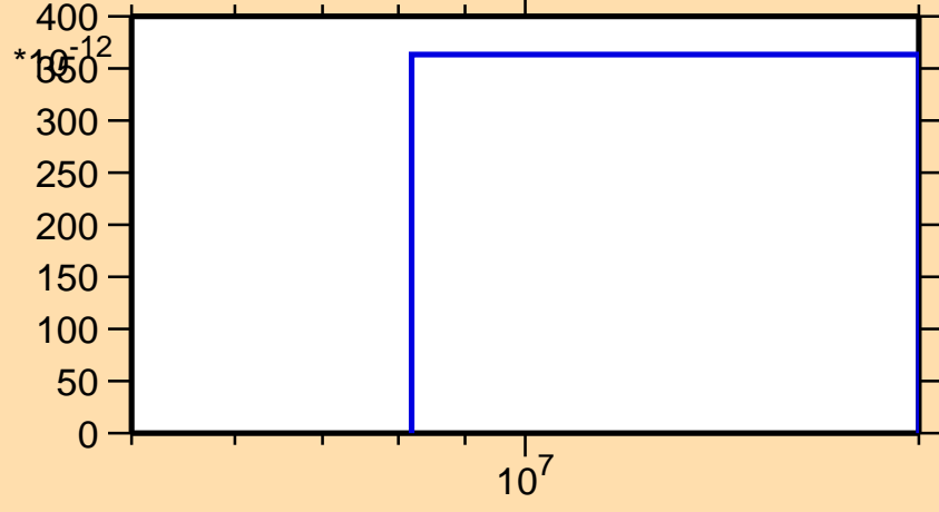
\sigma vs. E for ^{190}\text{Pb}(n,\text{nd})
