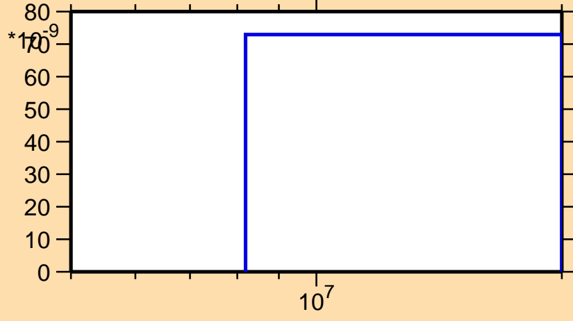
\sigma vs. E for ^{190}\text{Pb}(\text{mt } 45)
