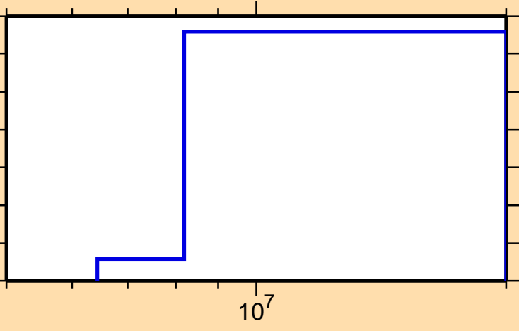
\sigma vs. E for ^{190}\text{Pb}(n,\text{He3})
