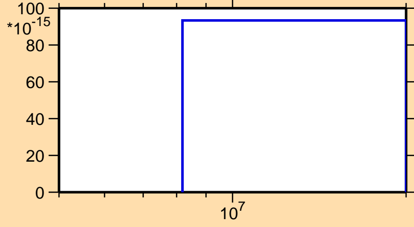
\sigma vs. E for ^{190}\text{Pb}(\text{mt } 34)
