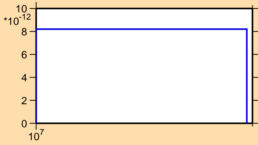
\sigma vs. E for ^{191}\text{Pb} (mt 34)
