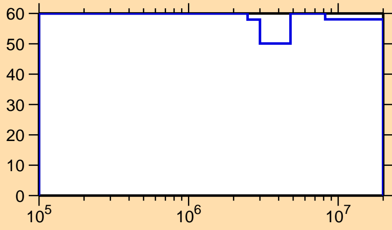
\Delta\sigma/\sigma vs. E for ^{191}\text{Pb}(n,n_1)
