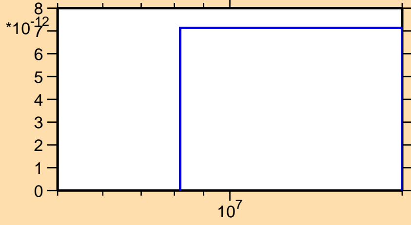
\sigma vs. E for ^{191}\text{Pb}(\text{mt } 34)
