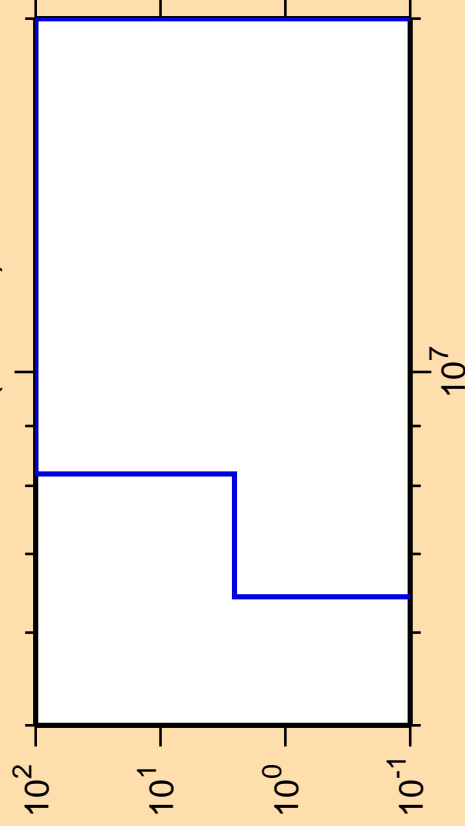
\Delta\sigma/\sigma vs. E for ^{191}\text{Pb}(n,\text{He}3)
