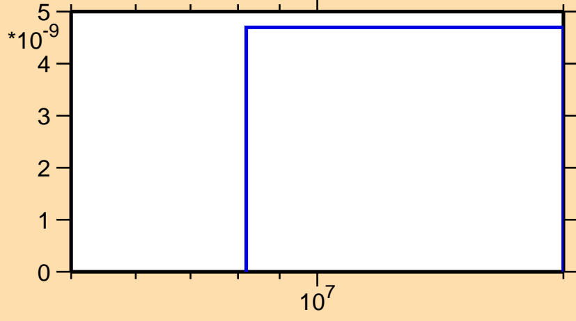
\sigma vs. E for ^{191}\text{Pb}(\text{mt } 45)
