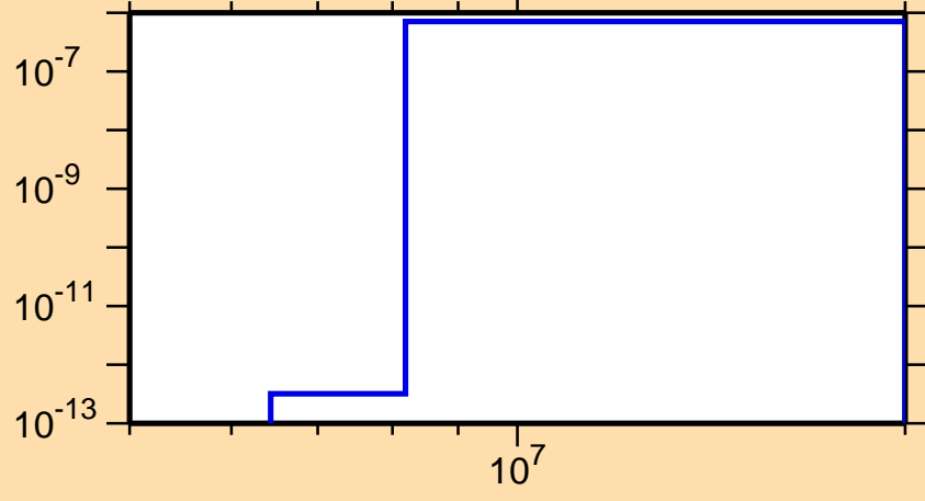
\sigma vs. E for ^{191}\text{Pb}(n,\text{He}3)
