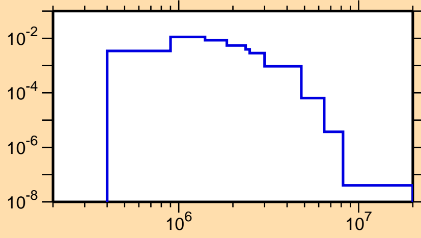
\sigma vs. E for ^{191}\text{Pb}(n,n_2)
