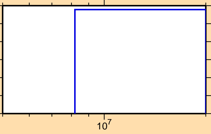
\sigma vs. E for ^{191}\text{Pb}(n,\text{pd})
