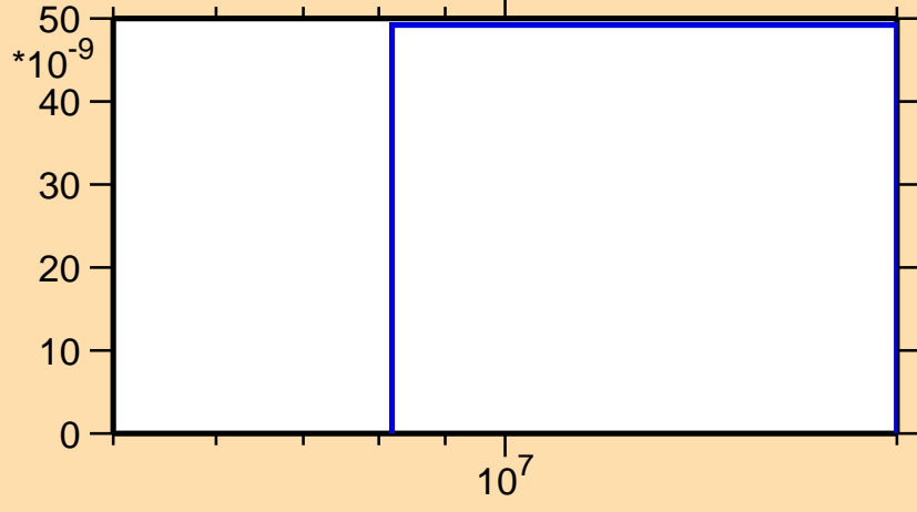
\sigma vs. E for ^{191}\text{Pb}(n,\text{nd})
