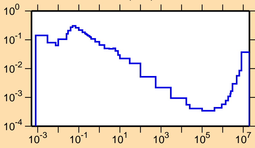
\sigma vs. E for ^{191}\text{Pb}(n,\alpha)
