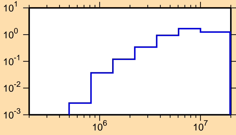
\sigma vs. E for ^{191}\text{Pb}(n,n\text{cont.})
