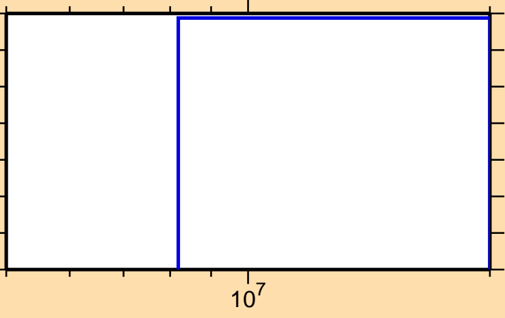
\sigma vs. E for ^{191}\text{Pb}(n,\text{nd})
