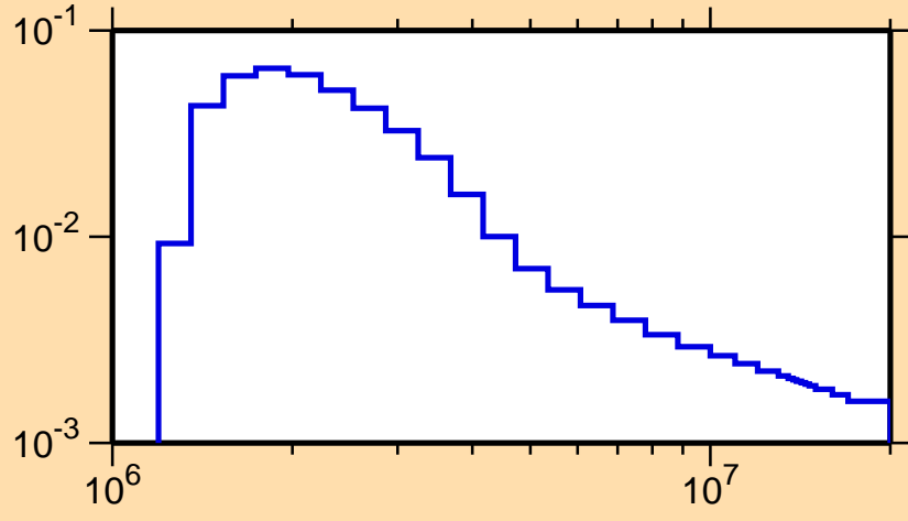
\sigma vs. E for ^{192}\text{Pb}(n,n_3)
