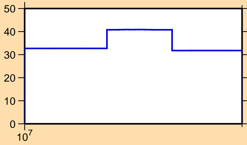
\Delta\sigma/\sigma vs. E for ^{192}\text{Pb}(n,\text{inel.})
