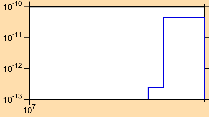
\sigma vs. E for ^{192}\text{Pb}(n,\text{pt})
