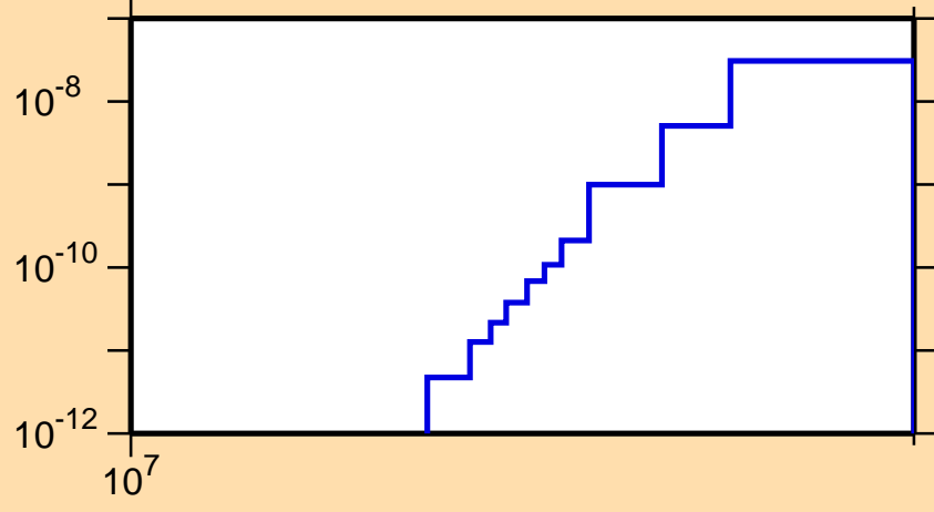
\sigma vs. E for ^{192}\text{Pb}(n,\text{pd})
