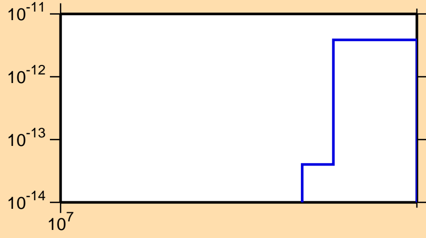
\sigma vs. E for ^{192}\text{Pb}(\text{mt } 34)
