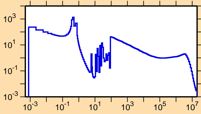
\sigma vs. E for ^{192}\text{Pb}(n,\gamma)
