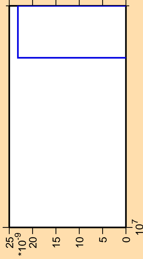
\Delta\sigma/\sigma vs. E for ^{192}\text{Pb}(\text{mt } 11)
