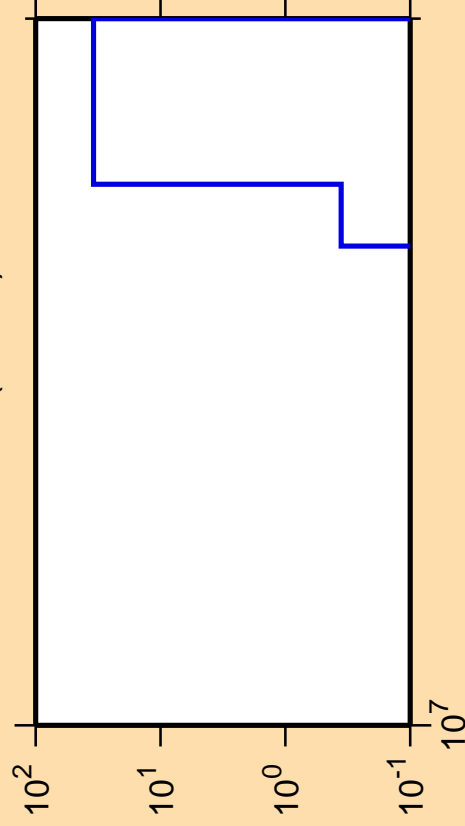
\Delta\sigma/\sigma vs. E for ^{192}\text{Pb}(\text{mt } 34)
