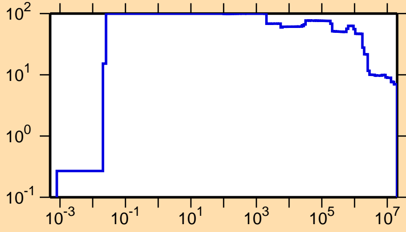
\Delta\sigma/\sigma vs. E for ^{192}\text{Pb}(n,\text{nonel.})
