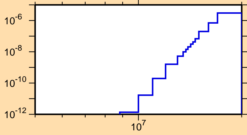
\sigma vs. E for ^{192}\text{Pb}(n,\text{He}3)
