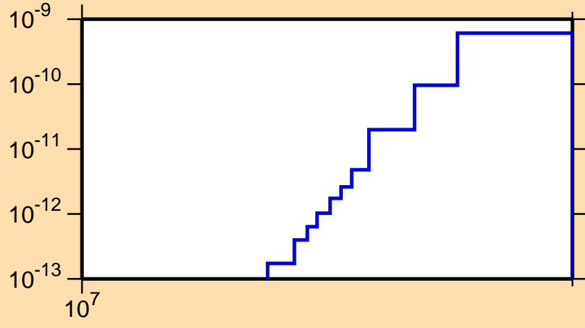
\sigma vs. E for ^{192}\text{Pb}(\text{mt117})
