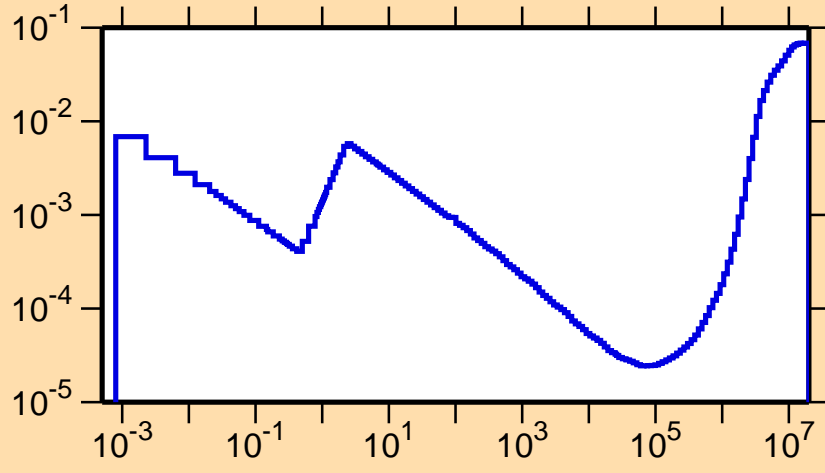
\sigma vs. E for ^{192}\text{Pb}(n,p)
