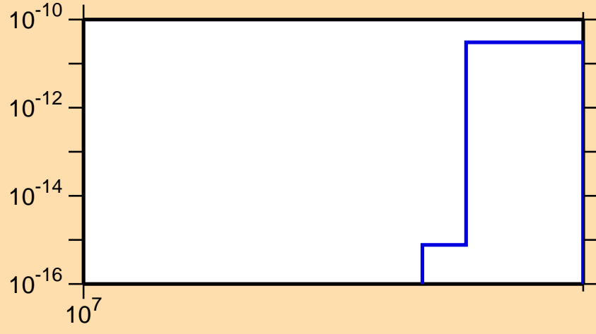
\sigma vs. E for ^{192}\text{Pb}(n,nt)
