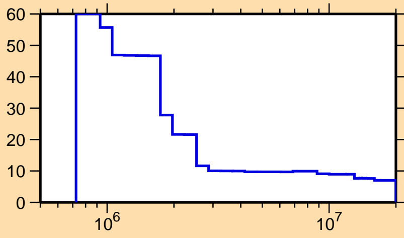
\Delta\sigma/\sigma vs. E for ^{192}\text{Pb}(n,\text{nonel.})
