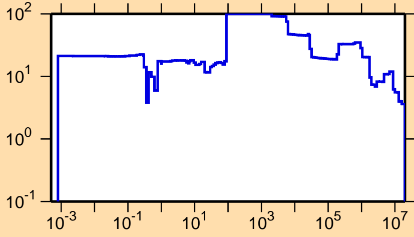
\Delta\sigma/\sigma vs. E for ^{192}\text{Pb}(n,\text{tot.})
