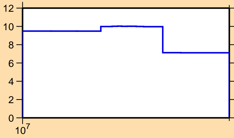
\Delta\sigma/\sigma vs. E for ^{192}\text{Pb}(n,\text{el.})
