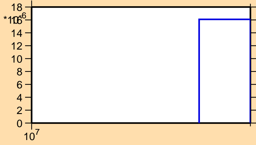
\sigma vs. E for ^{192}\text{Pb}(n,3n)
