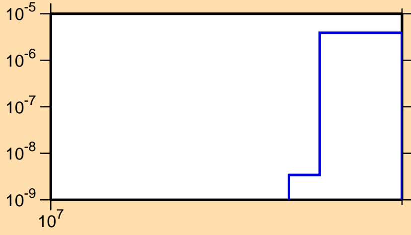
\sigma vs. E for ^{192}\text{Pb}(n,2np)
