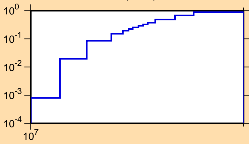
\sigma vs. E for ^{192}\text{Pb}(n,2n)
