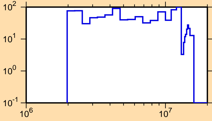
\Delta\sigma/\sigma vs. E for ^{192}\text{Pb}(n,n_1)
