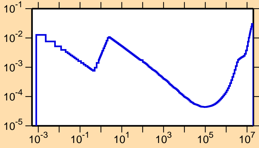
\sigma vs. E for ^{192}\text{Pb}(n,\alpha)
