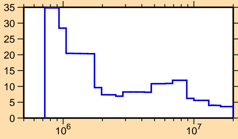
\Delta\sigma/\sigma vs. E for ^{192}\text{Pb}(n,\text{tot.})
