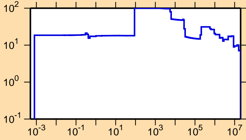
\Delta\sigma/\sigma vs. E for ^{192}\text{Pb}(n,\text{el.})
