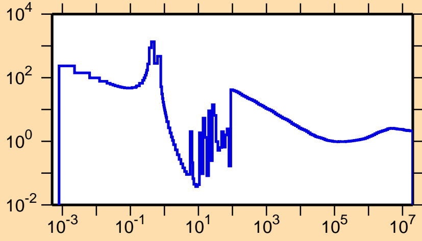
\sigma vs. E for ^{192}\text{Pb}(n,\text{nonel.})
