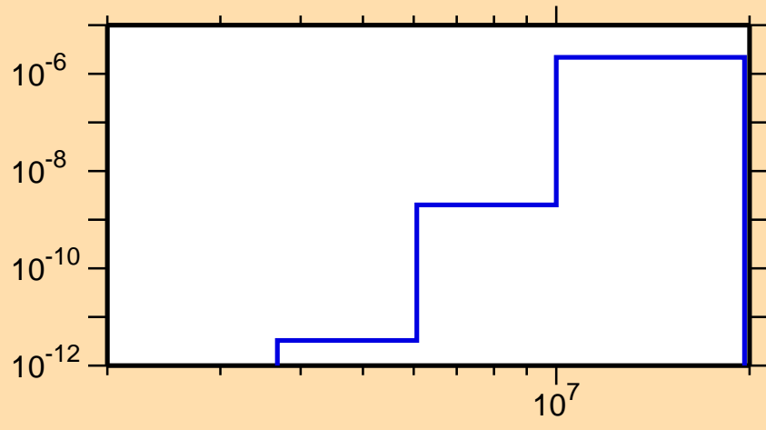
\sigma vs. E for ^{192}\text{Pb}(n,p\alpha)
